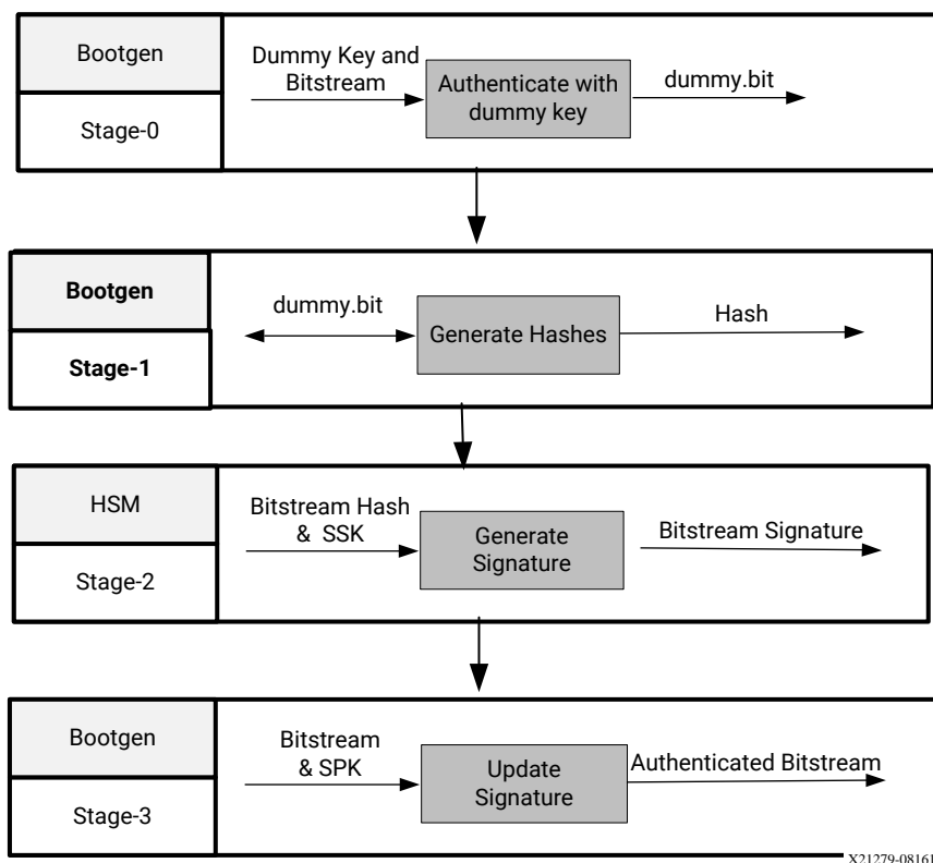
Figure 23: HSM Mode Flow
