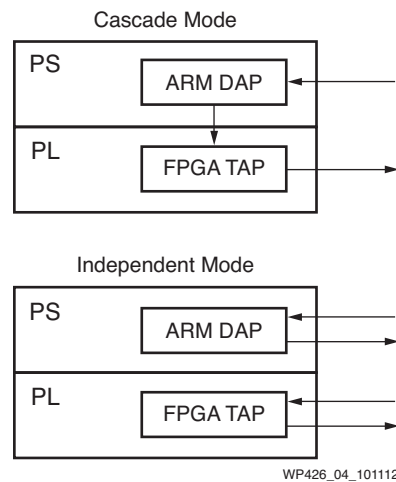
Figure 3: Debug-JTAG Chain
