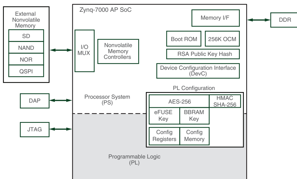
Figure 1: Zynq-7000 AP SoC Security Architecture
