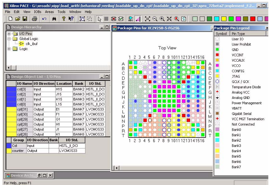
Figure 3: Pin Assignment in Xilinx PACE™ Tool
