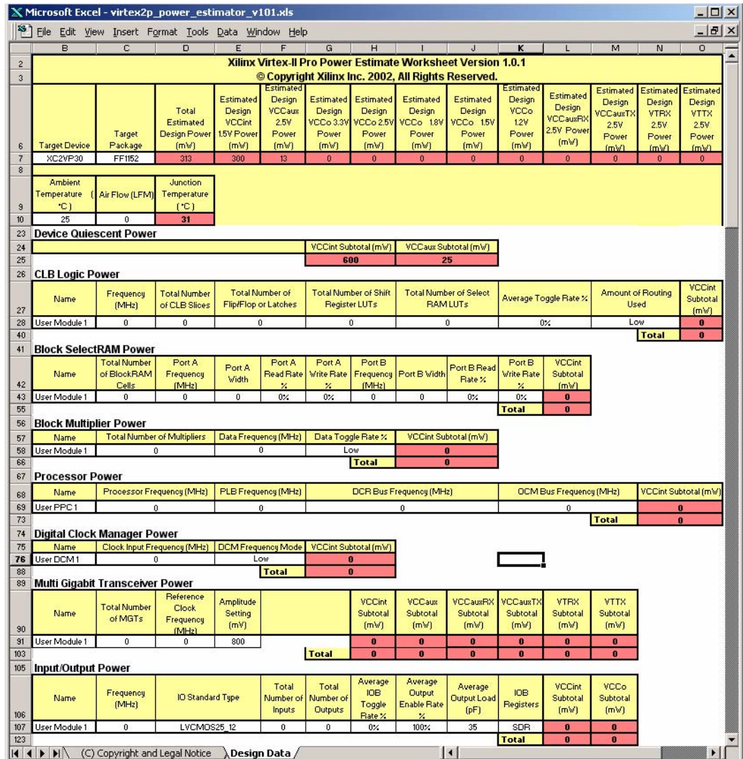
Figure 5: Pre-Implementation Power Estimation Spreadsheets for the Different Xilinx Device Families
