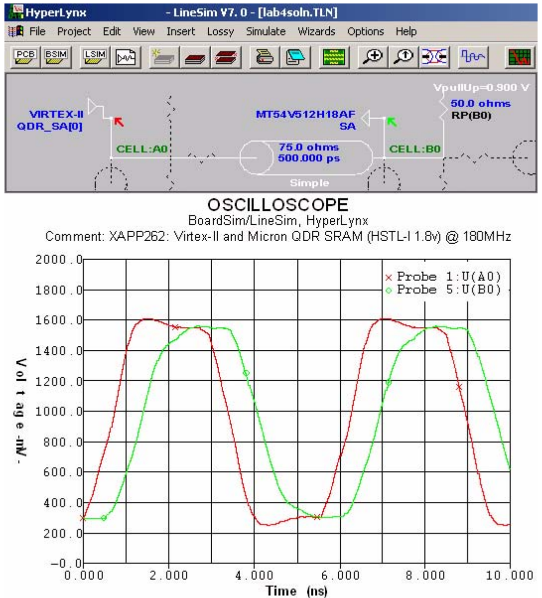
Figure 8: Pre-Layout SI Analysis Using Mentor’s HyperLynx™ Suite
