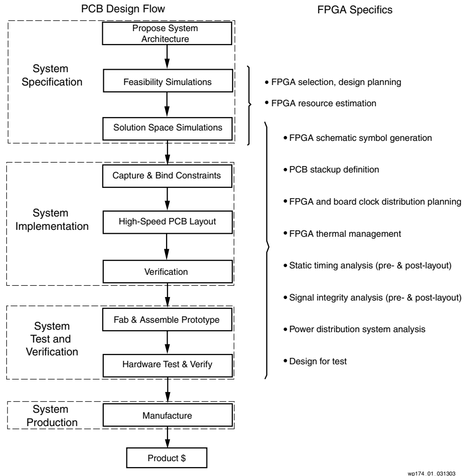
Figure 1: High-Speed PCB Design Flow and FPGA Specifics
