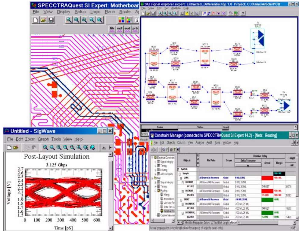
Figure 9: Post-Layout SI Analysis Example Using Cadence® SPECCTRAQuest™
