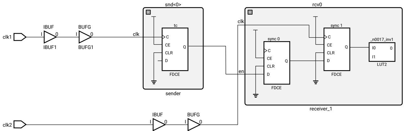
Figure 45: Synchronizing Clock Domains
