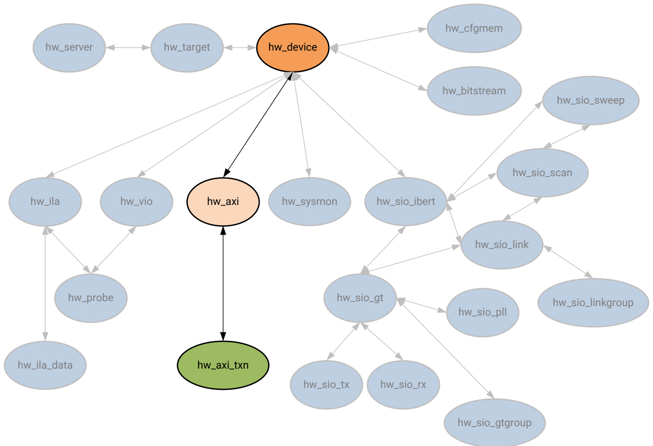
Figure 18: Hardware AXI Objects
