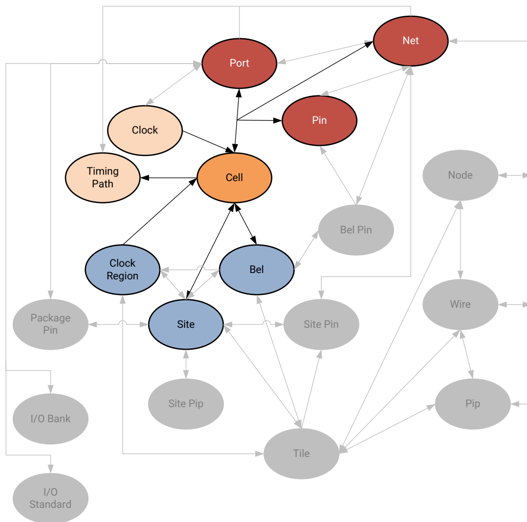
Figure 15: CELL Objects
