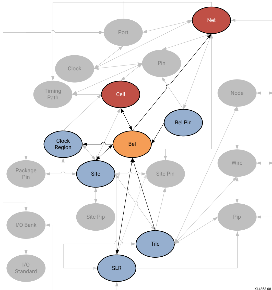
Figure 13: BEL Objects
