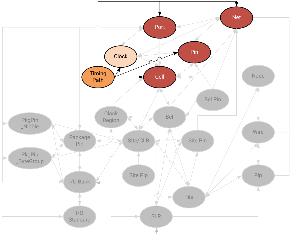
Figure 43: TIMING_PATH Objects
