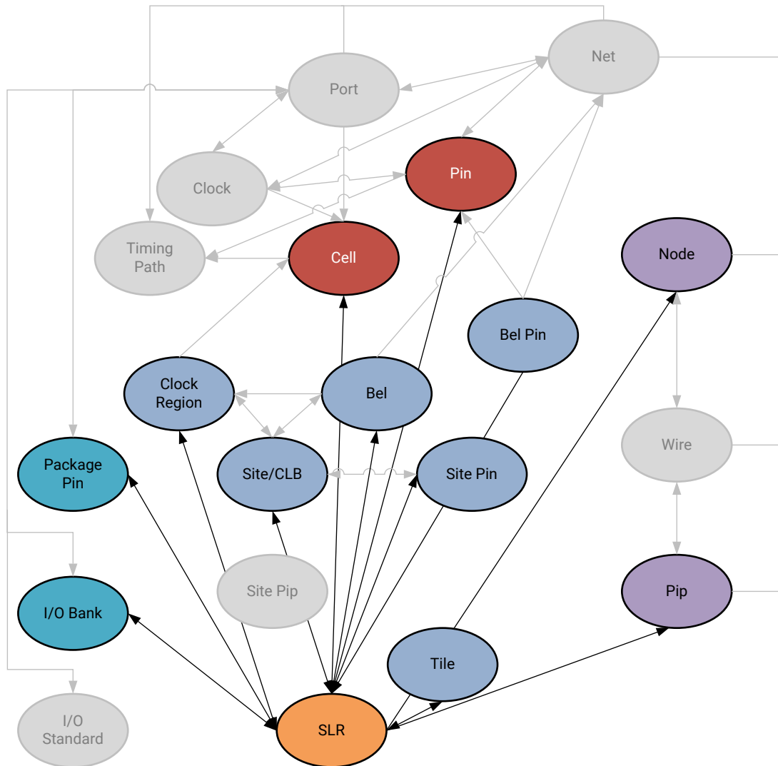
Figure 41: SLR Objects
