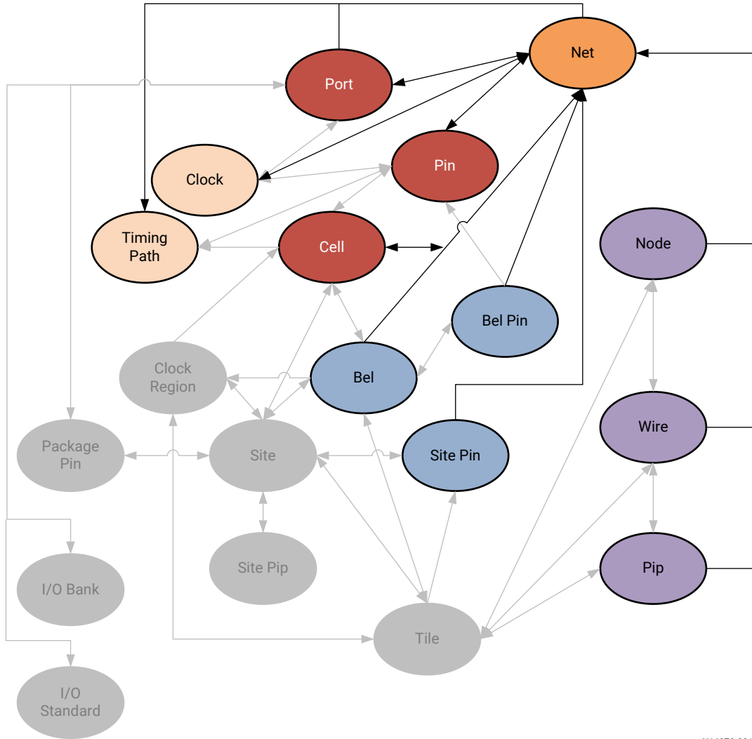
Figure 32: NET Objects
