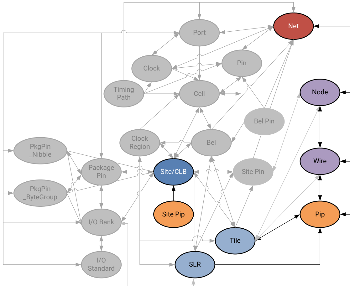
Figure 36: PIP Objects
