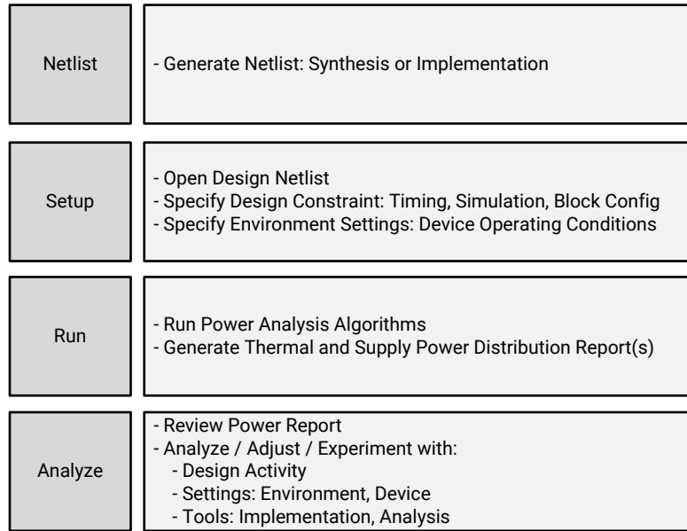
Figure 17: Power Analysis Flow
