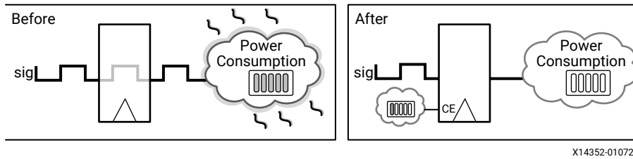
Figure 29: Intelligent Clock Gating
