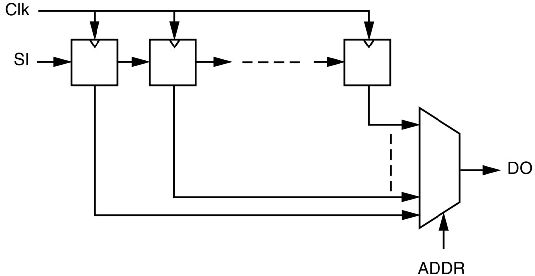
Figure 4-1: Dynamic Shift Registers Diagram
