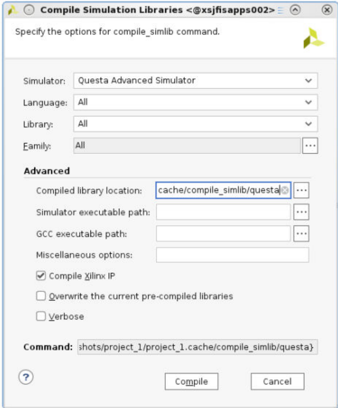
Figure 2: Compile Simulation Libraries Dialog Box
