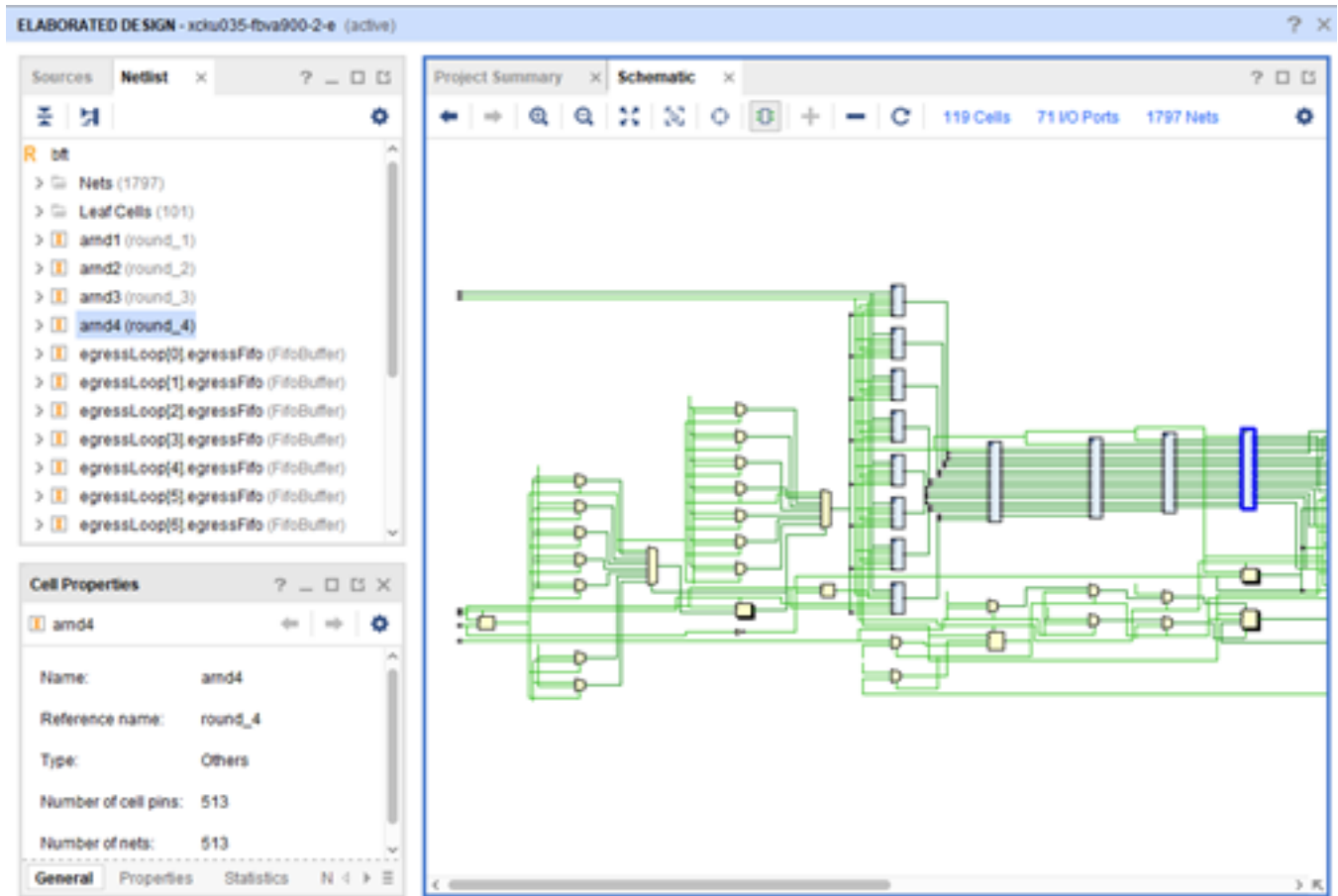
Figure 47: Elaborated Design in the RTL Schematic Window
