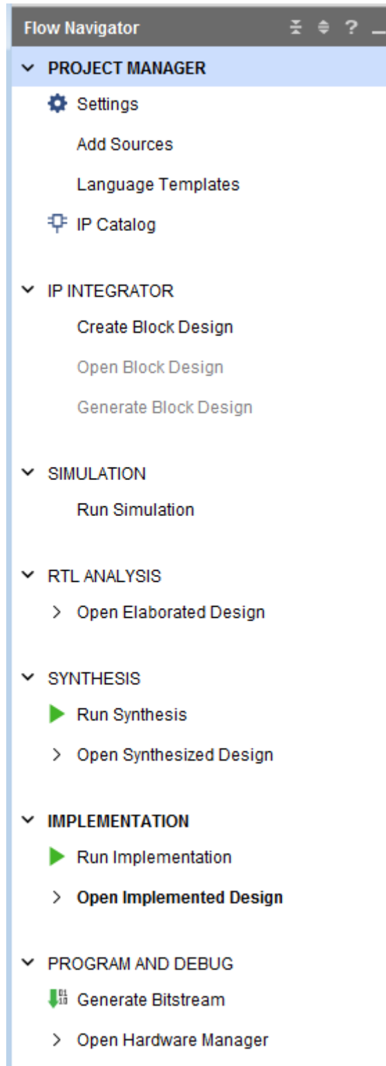
Figure 8: Flow Navigator
