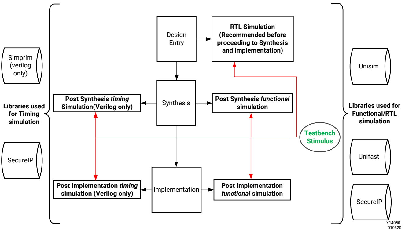
Figure 15: Simulation at Various Points in the Design Flow
