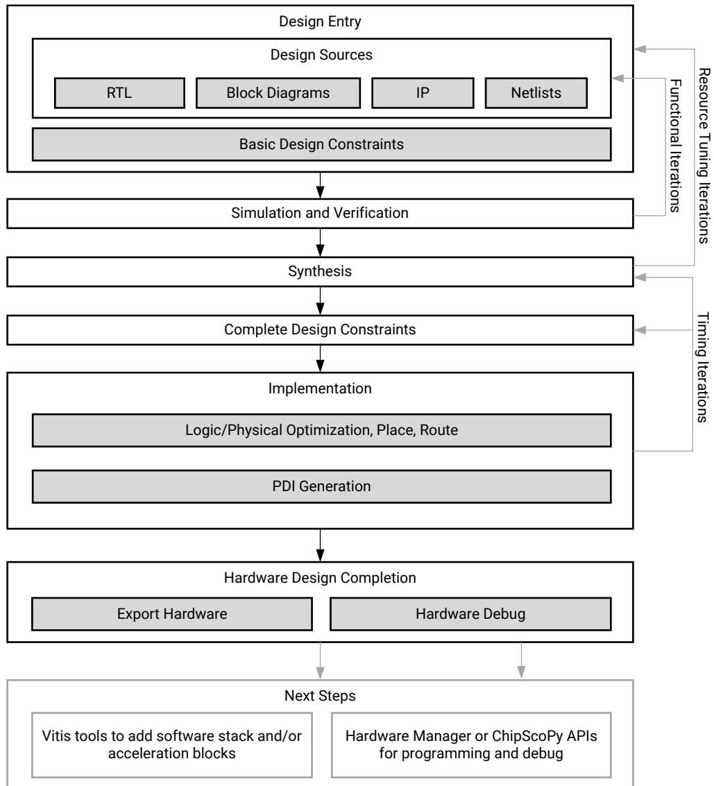
Figure 2: Traditional Design Flow for Versal Devices
