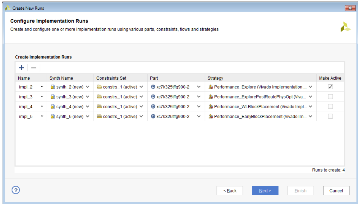
Figure 16: Creating Multiple Synthesis and Implementation Runs
