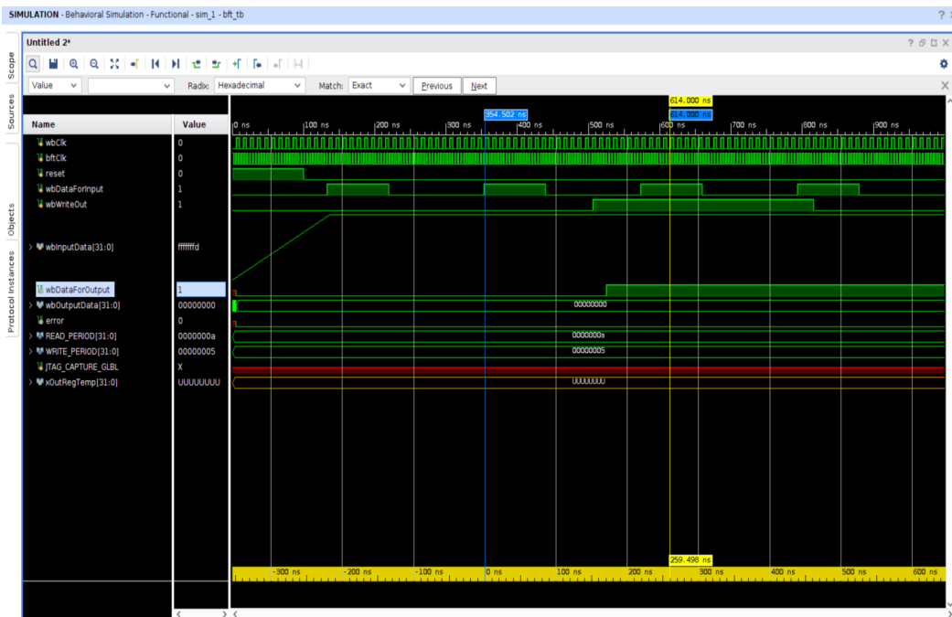
Figure 16: Wave Window
