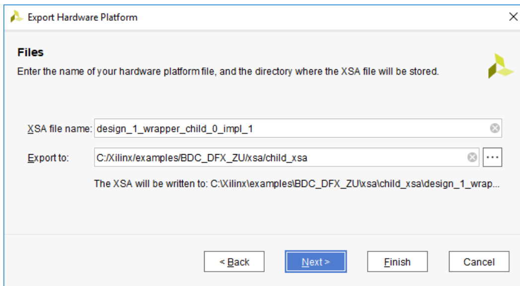
Figure 141: Export the Hardware Platform for the Child Configuration
