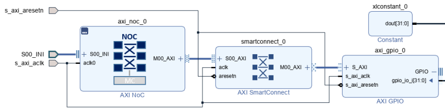
Figure 161: Completed RM2 Block Design
