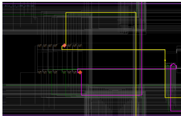
Figure 92: Magnified View of Device. Top Half of RCLK is Used by One Partition's Clock Net And Bottom Half is Used By Other Partition's Clock Net
