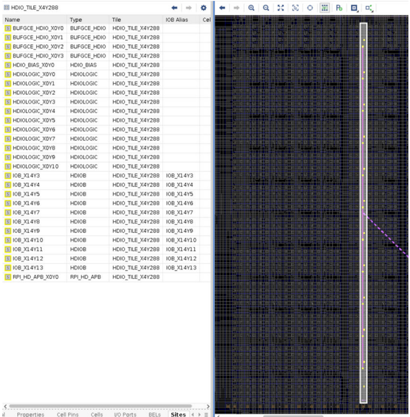
Figure 89: Clock Buffers and IOB in HDIO Bank Share Same PU: HDIO_TILE
