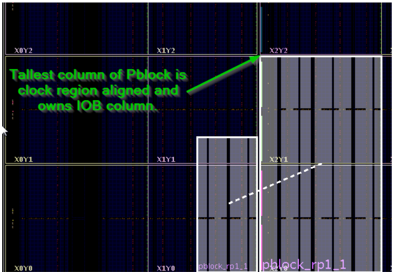
Figure 69: Tallest Column of Pblock Clock Region Aligned
