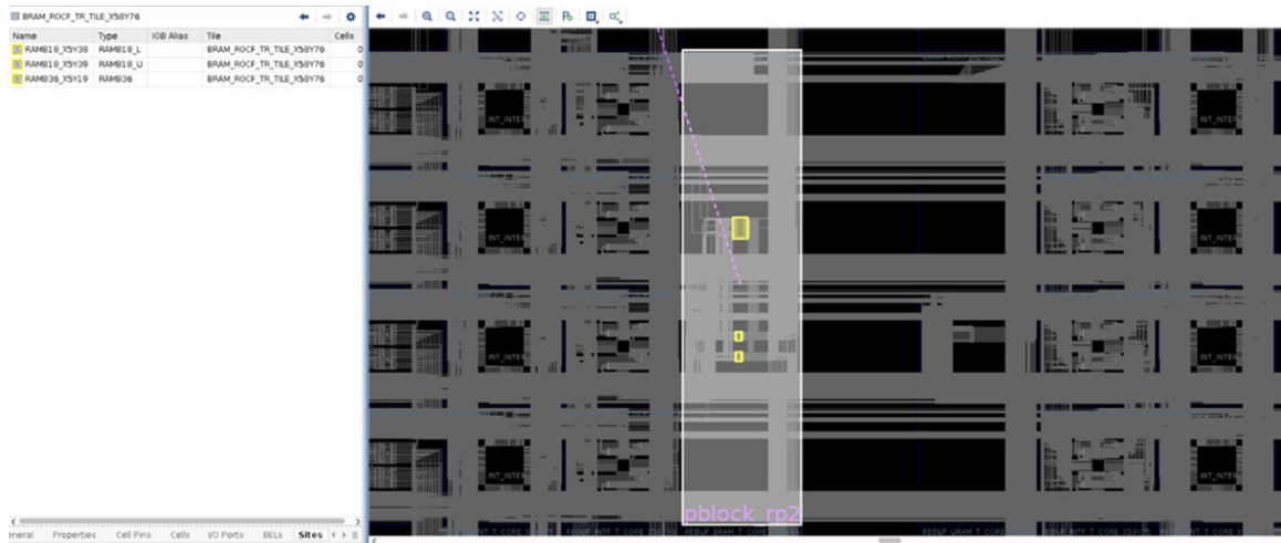
Figure 73: BRAM PU: RAMB18s and RAMB36 of 1 BRAM Tile
