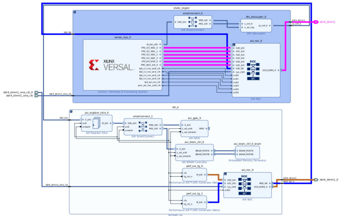
Figure 107: Hardened DDR Memory Controllers
