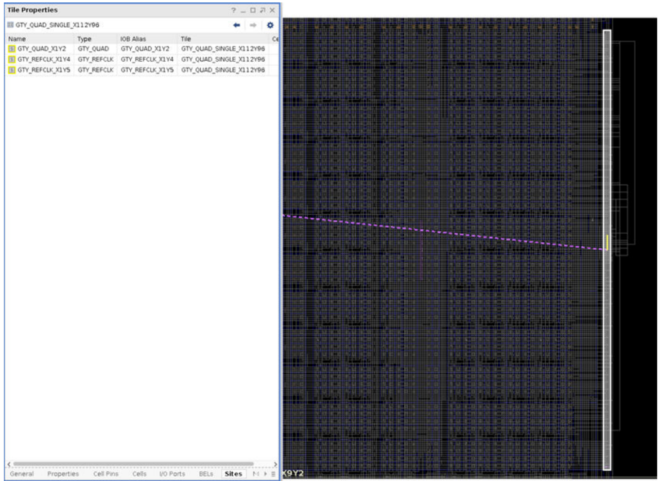
Figure 78: GTY_QUAD PU is GTY_QUAD Tile
