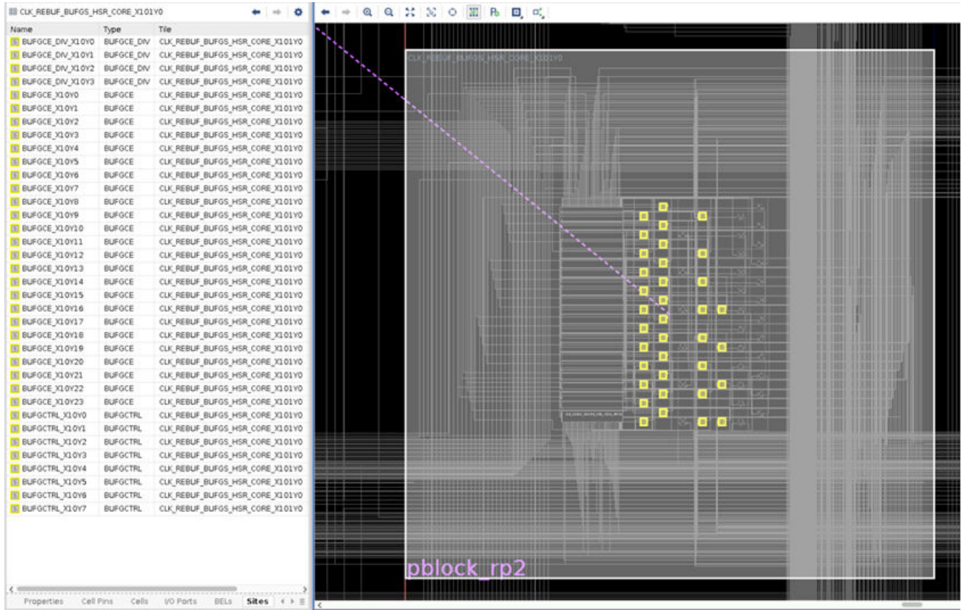
Figure 88: Clocking Buffers in HSR Has CLK_REBUF_BUFGRS_HSR_CORE Tile As PU
