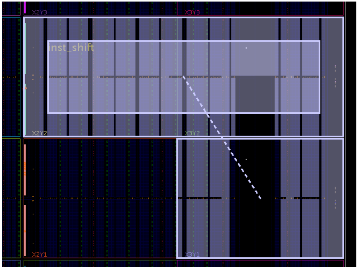
Figure 65: CLOCK_ROOT Restrictions on L-Shaped Pblocks
