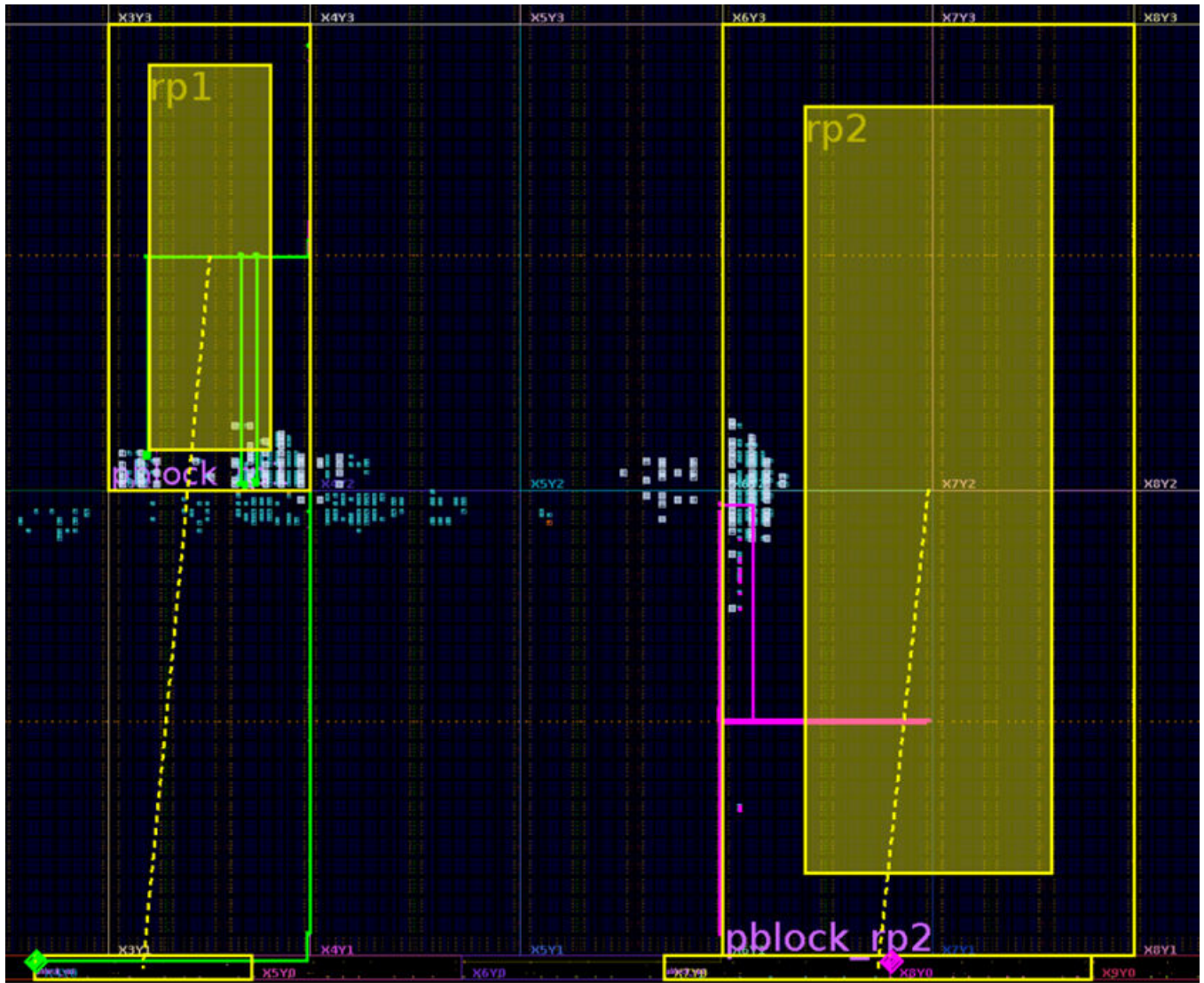
Figure 95: Clock Routing Expansion
