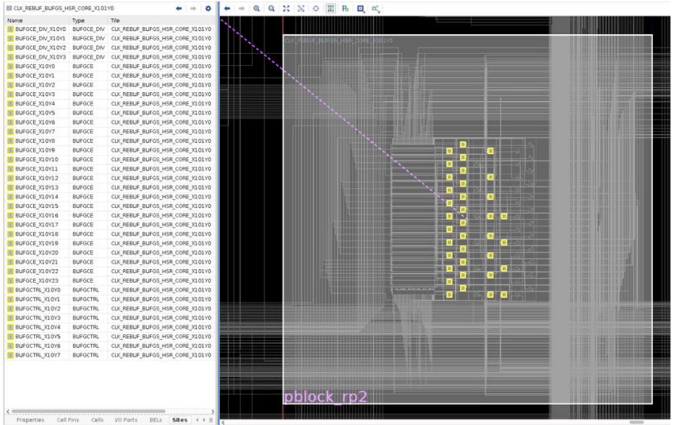
Figure 86: BUFGE_GT, BUFGE_SYNC Share Same PU: CLK_GT Tile
