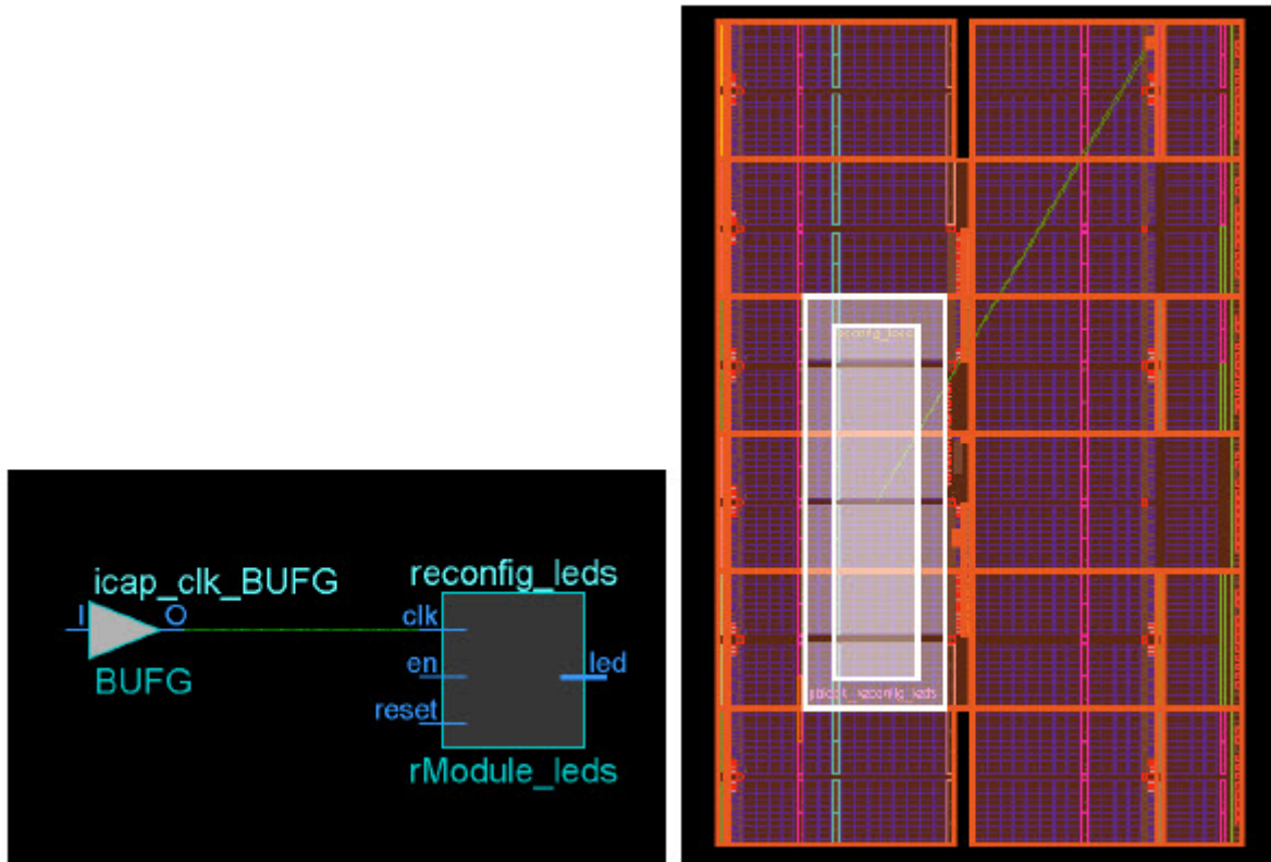
Figure 54: Pre-routing Global Clock to Reconfigurable Partition
