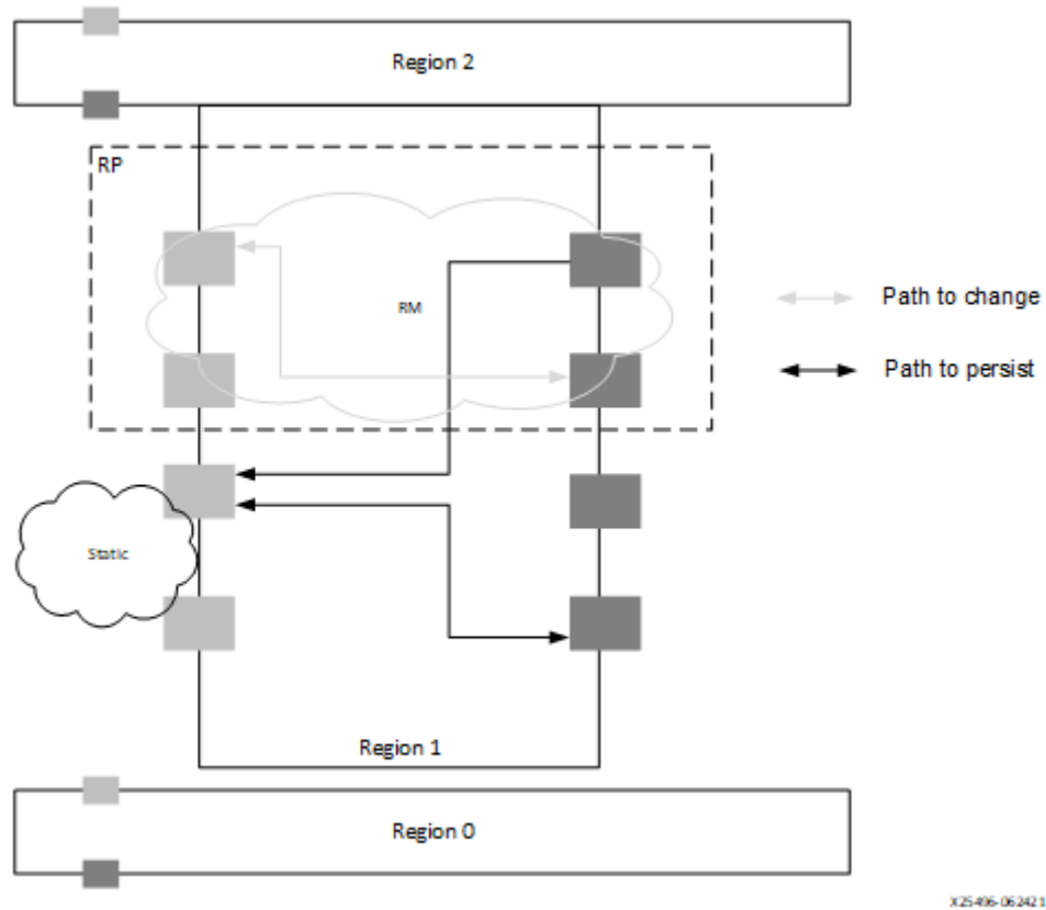
Figure 101: Part of the NoC in the RP, With Connections to Static NoC
