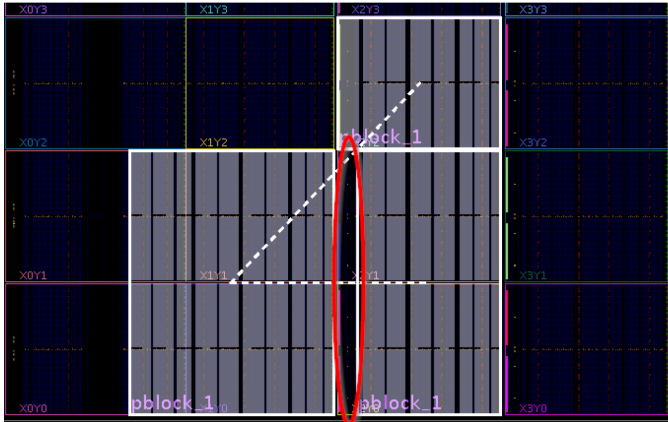
Figure 70: Unsupported Gap in the IOB Column
