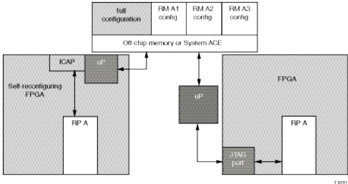
Figure 110: Configuring Through a Microprocessor
