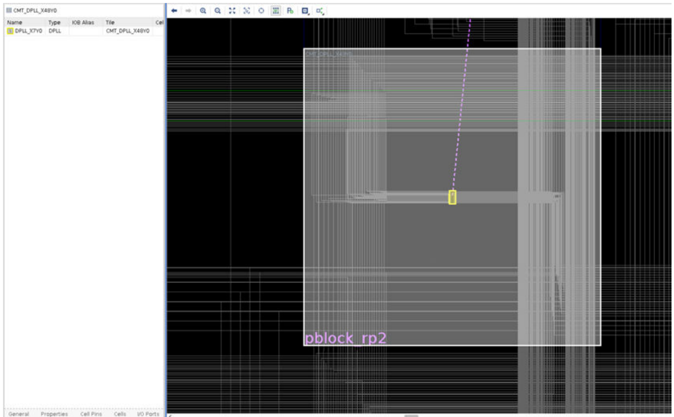
Figure 83: DPLL PU is CMT_DPLL Tile
