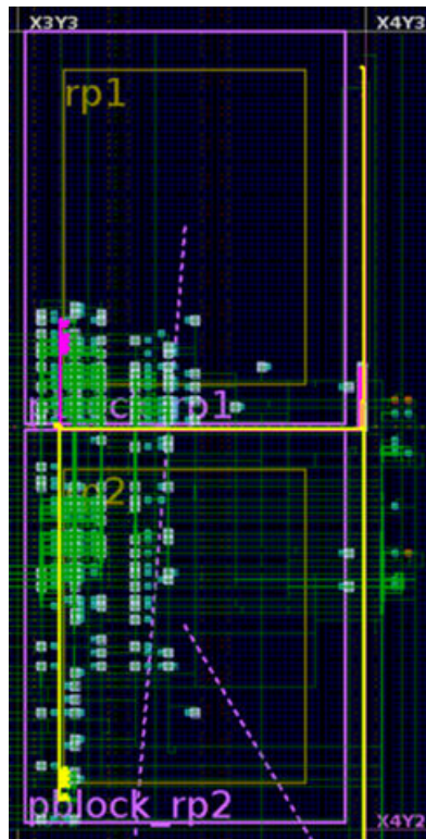
Figure 90: Sharing Clock Region between Multiple Reconfigurable Pblocks
