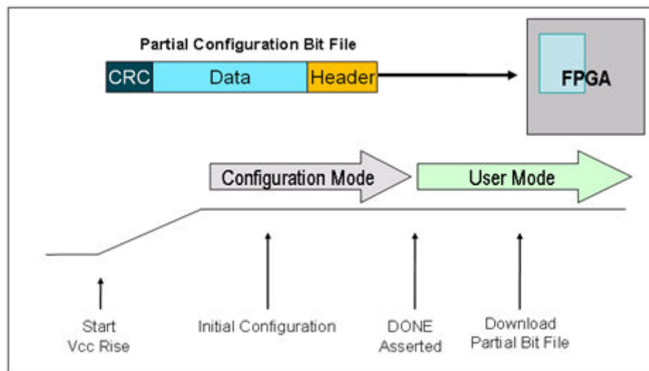
Figure 109: Configuring with a Partial BIT File
