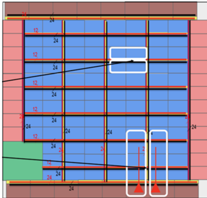
Figure 97: Clock Tile Partition
