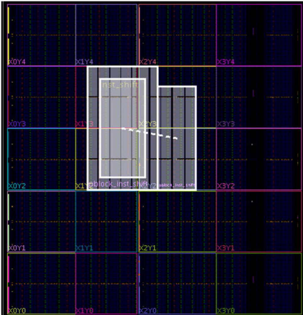
Figure 68: Supported Stair-Step Shaped Pblock
