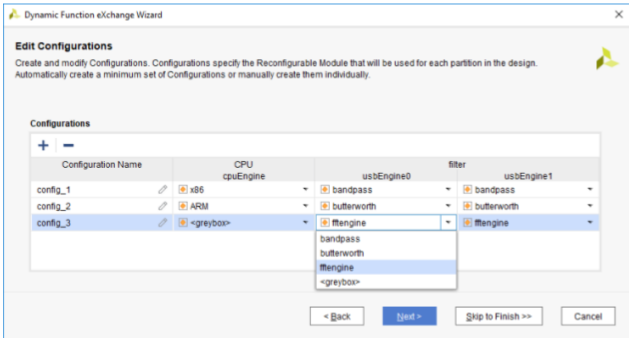
Figure 26: Edit Configurations after Automatic Generation of Configurations
