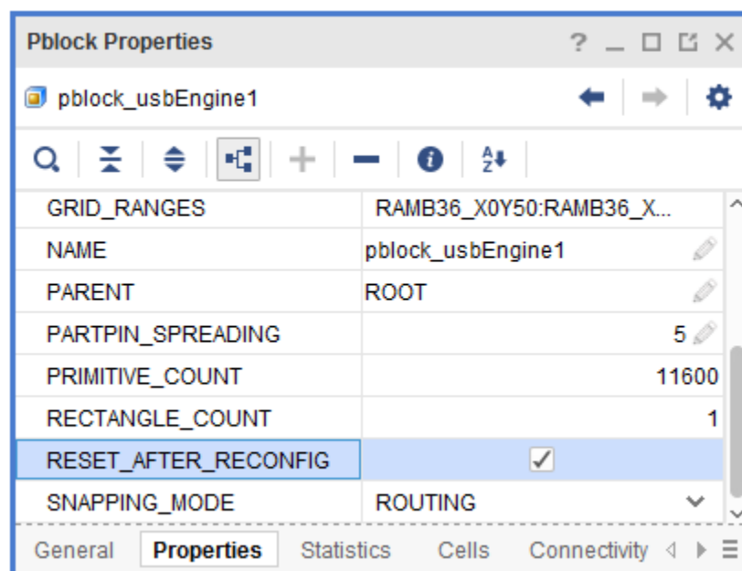
Figure 35: Dynamic Function eXchange Properties on a Pblock (7 series)
