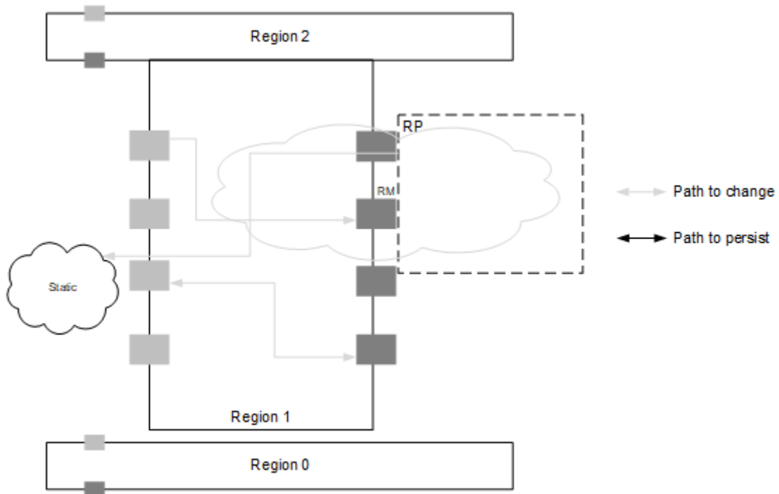
Figure 106: NoC Completely in an RP
