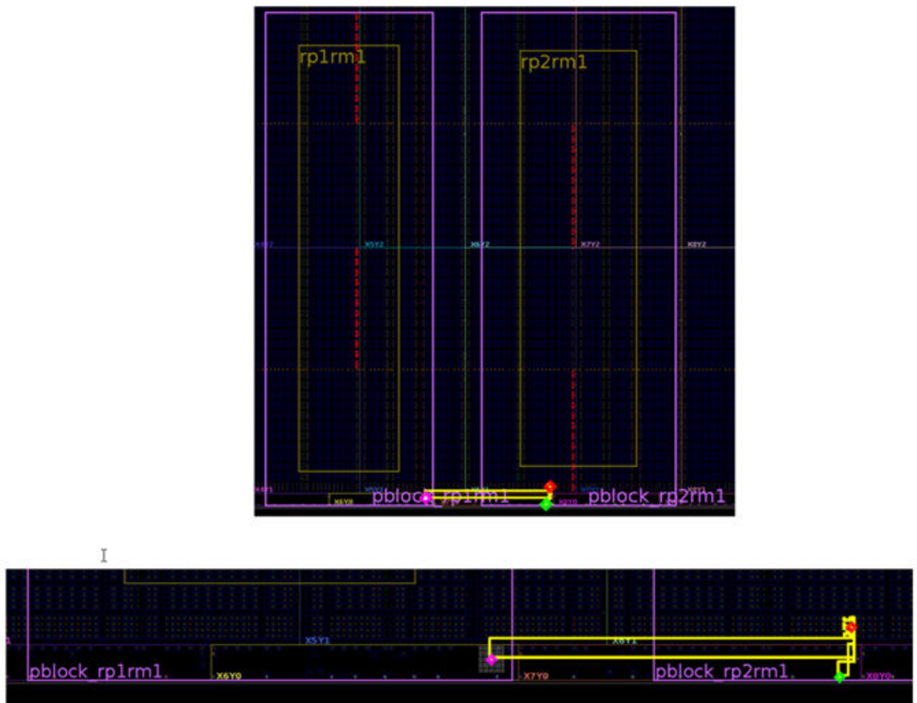
Figure 93: BLI Sharing and Floorplan Alignment
