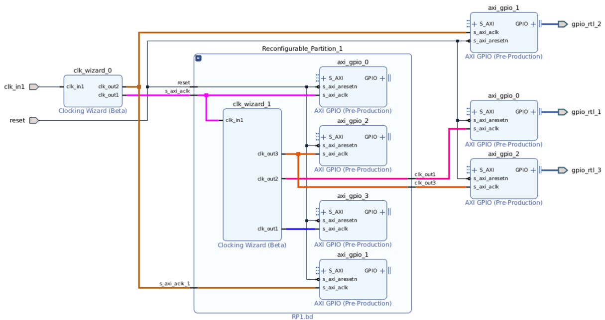
Figure 96: DFX Design Clocks
