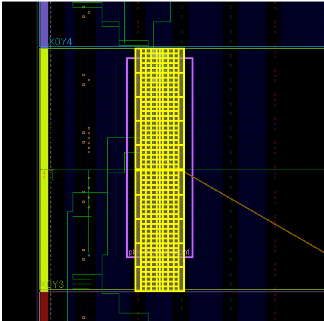
Figure 56: Original and Derived Pblocks Using SNAPPING_MODE
