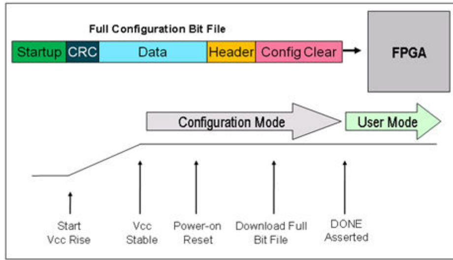
Figure 108: Configuring with a Full BIT File
