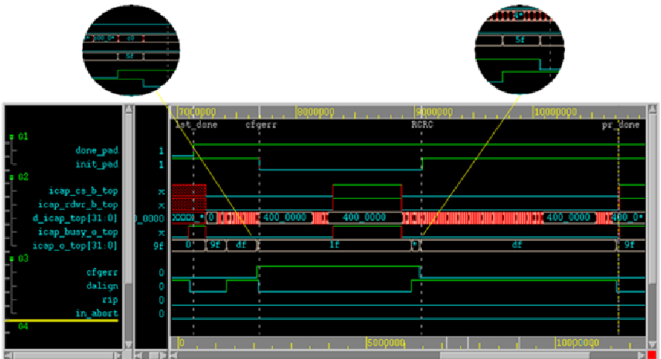
Figure 111: Vivado Logic Analyzer Display for Dynamic Function eXchange
