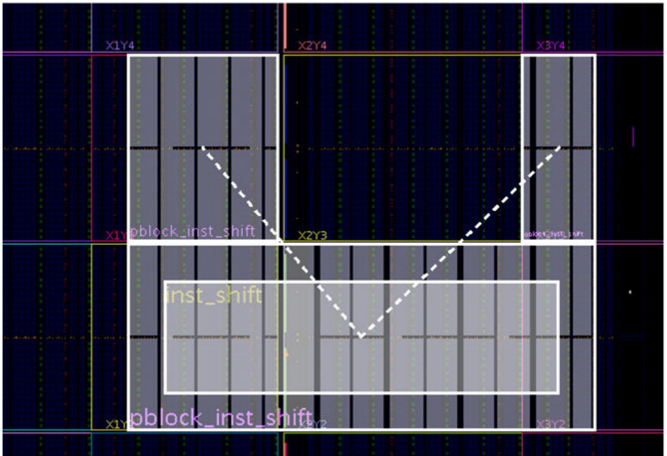
Figure 66: Unsupported Pblock with clock_region Gap
