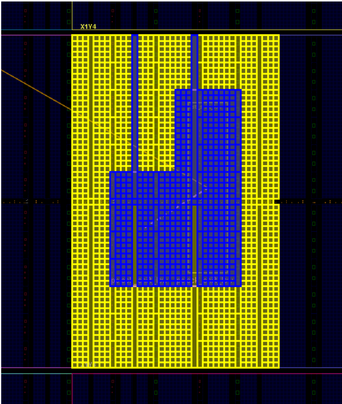
Figure 64: Highlighted Pblock and Expanded Routing Footprint
