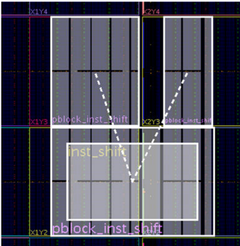
Figure 67: Supported Pblock with Small Static Gap
