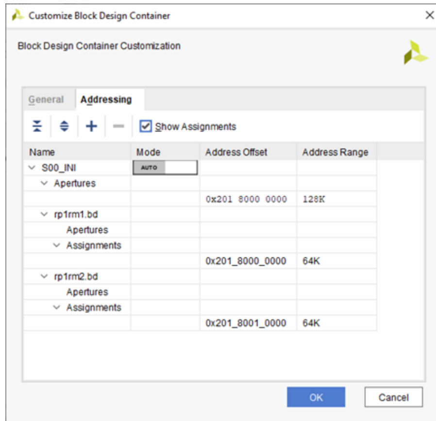
Figure 45: Viewing the Address Aperture for a BDC
