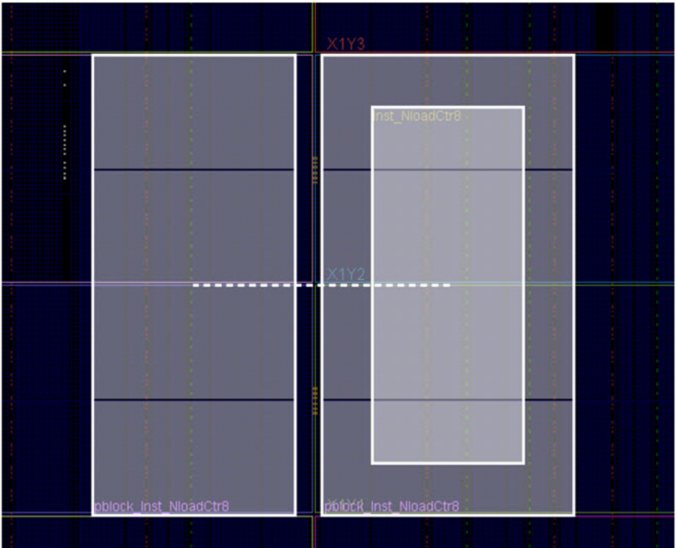
Figure 60: Multiple Pblock Rectangles that Avoid Non-Reconfigurable Resources
