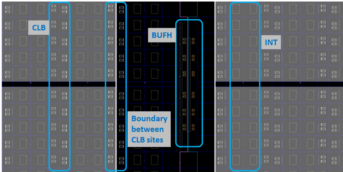
Figure 61: Close-up Showing Columns Reserved for Clock Routing Usage
