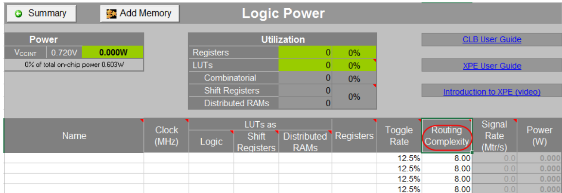
Figure 15: Routing Complexity in Logic Power Sheet for UltraScale Devices
