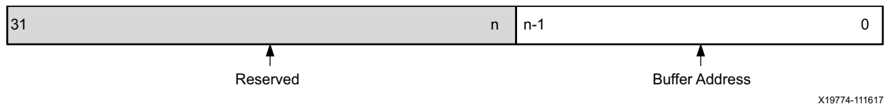
Figure 2-39: Profiling Buffer Address Register
