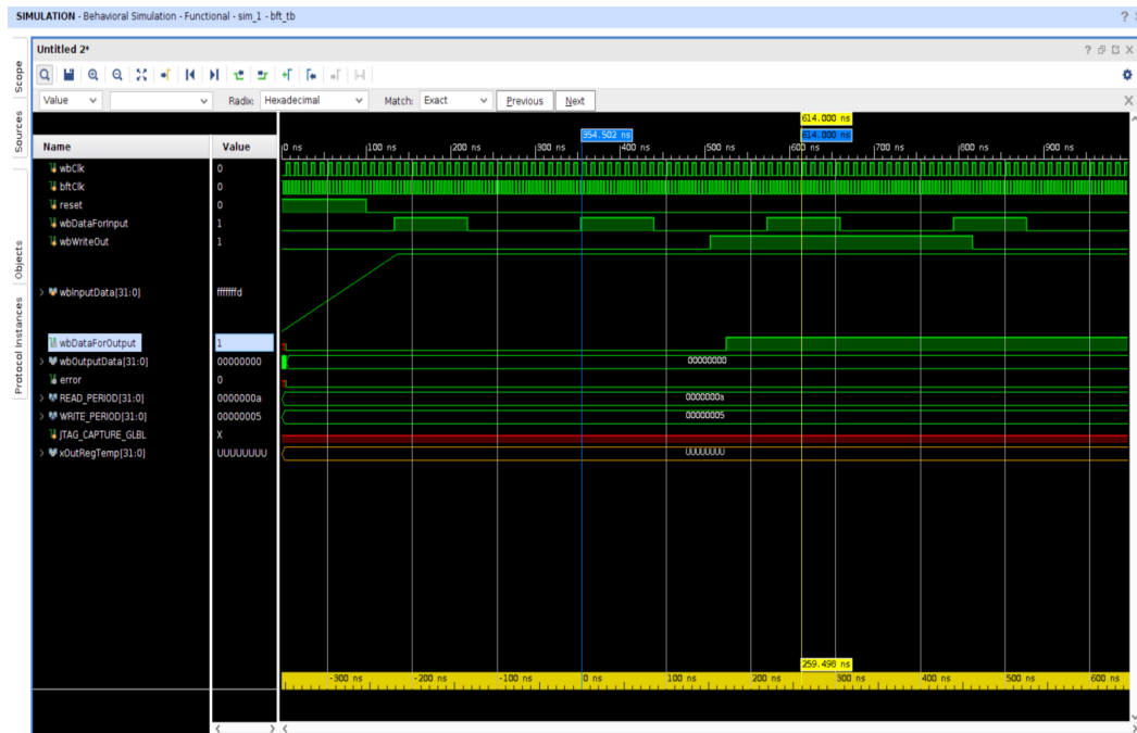
Figure 16: Wave Window
