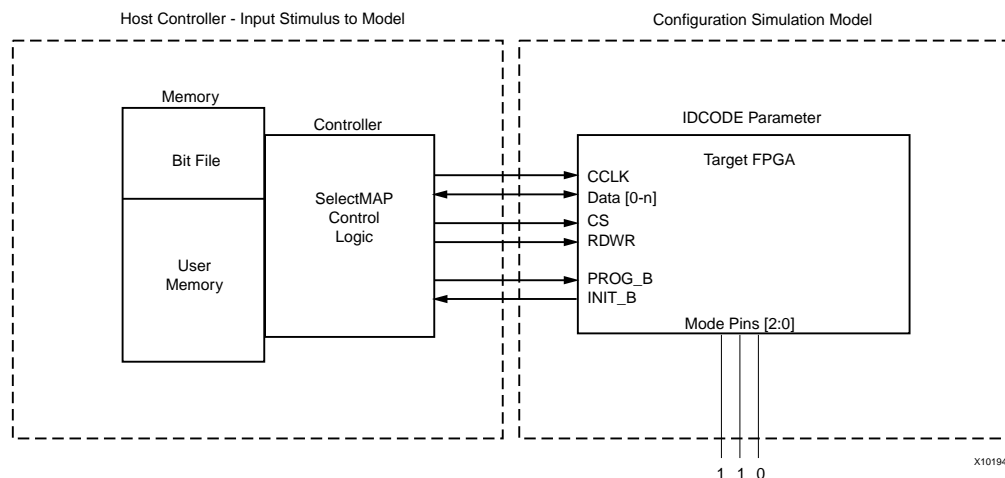
Figure 54: Block Diagram of Model Interaction
