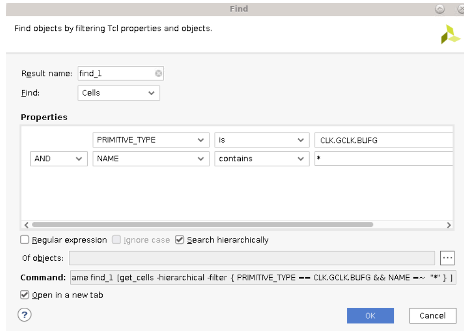
Figure 13: Finding Unplaced BUFGs
