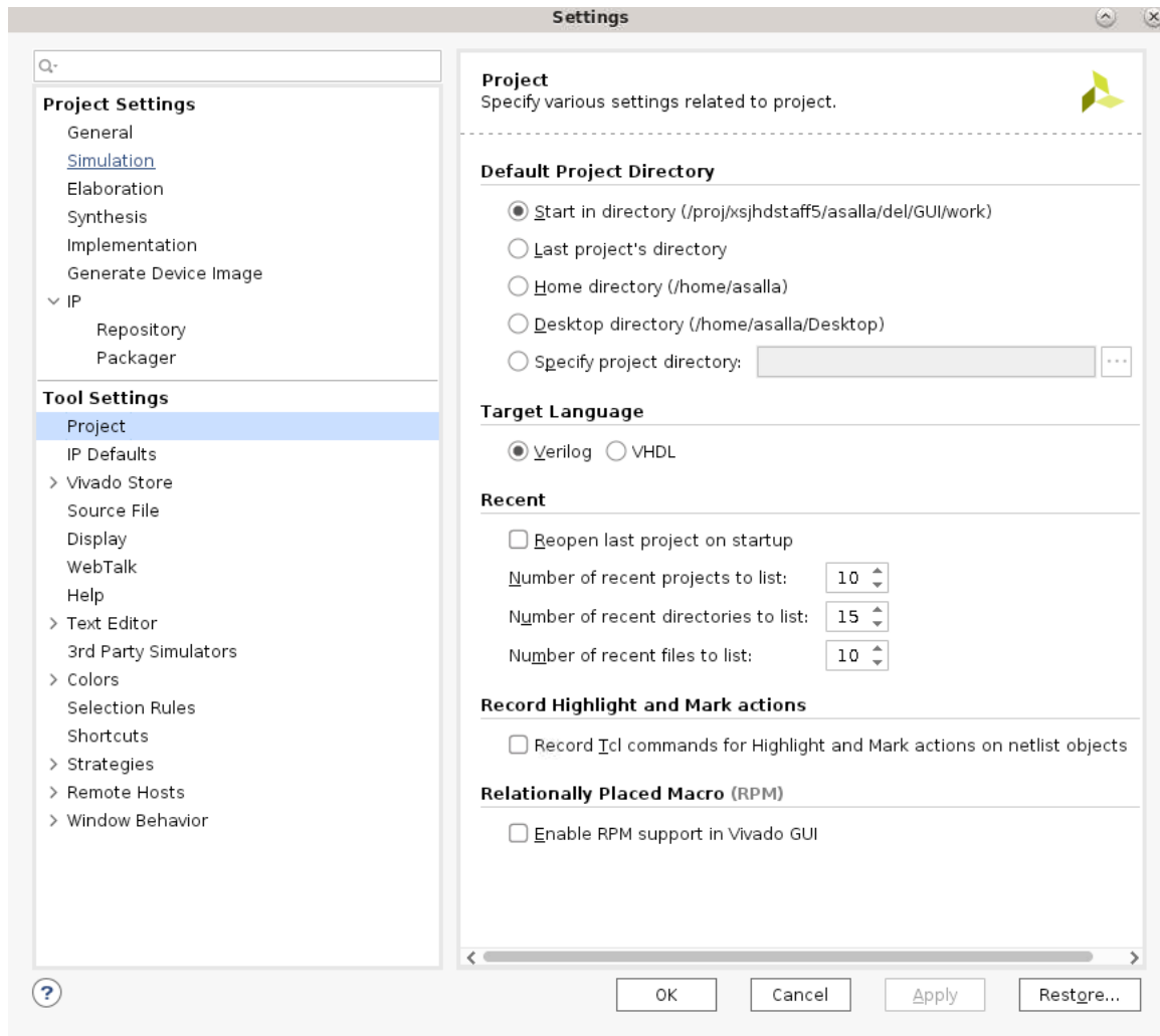
Figure 78: Settings Dialog Box—Tool Settings Project Category
