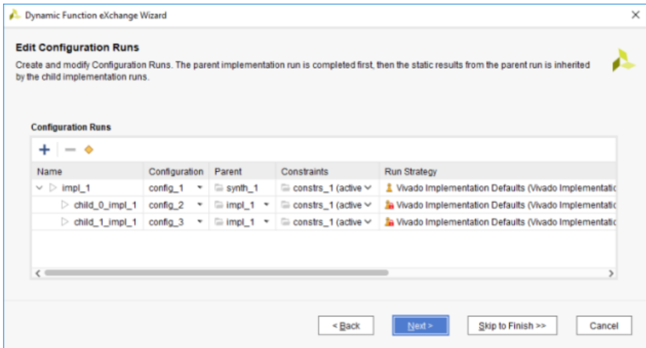
Figure 31: Automatically Generated Configuration Runs
