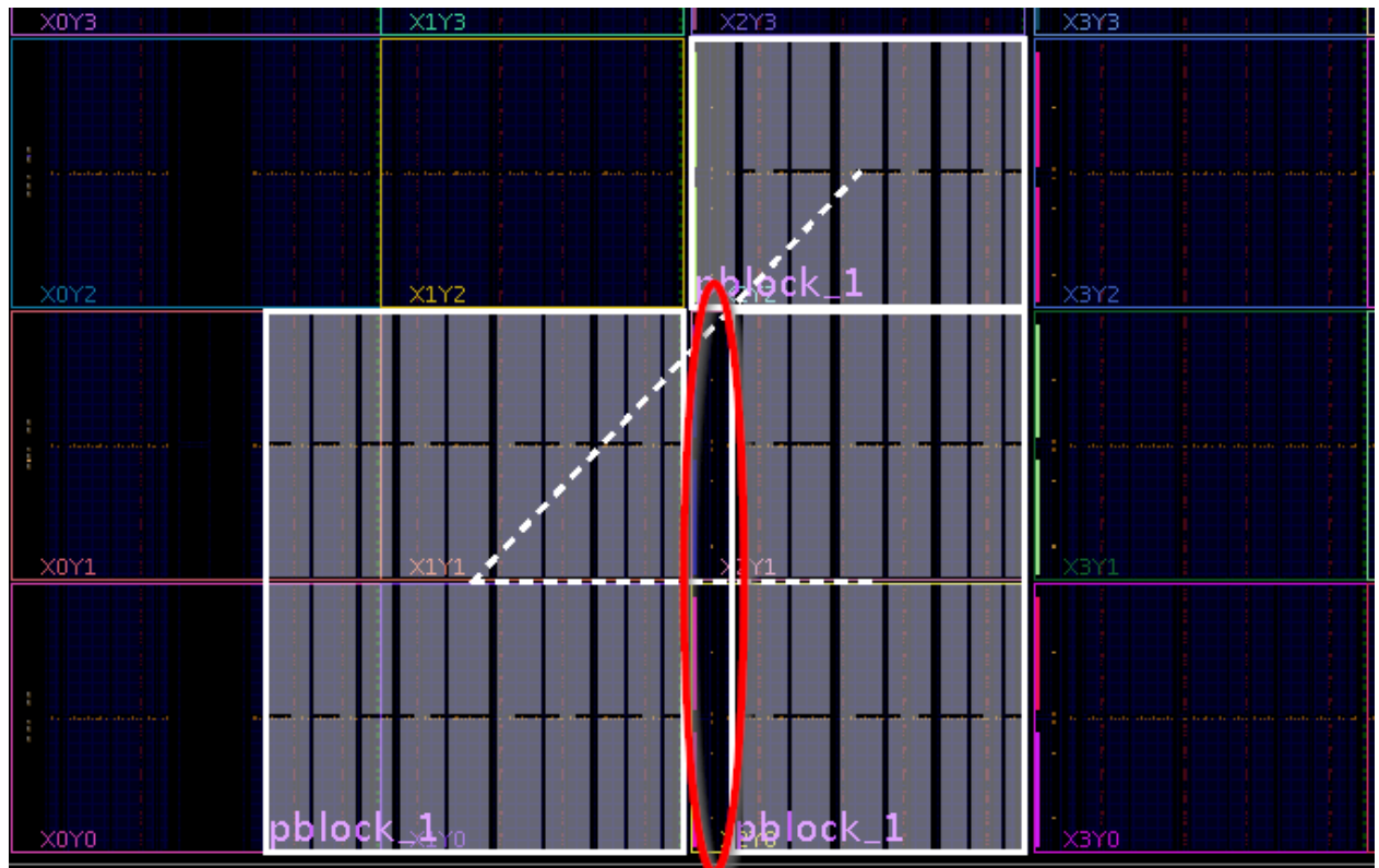
Figure 59: Unsupported Gap in the IOB Column
