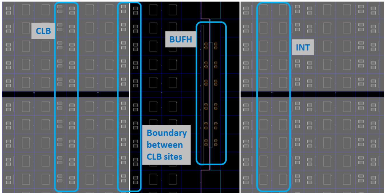
Figure 50: Close-up Showing Columns Reserved for Clock Routing Usage
