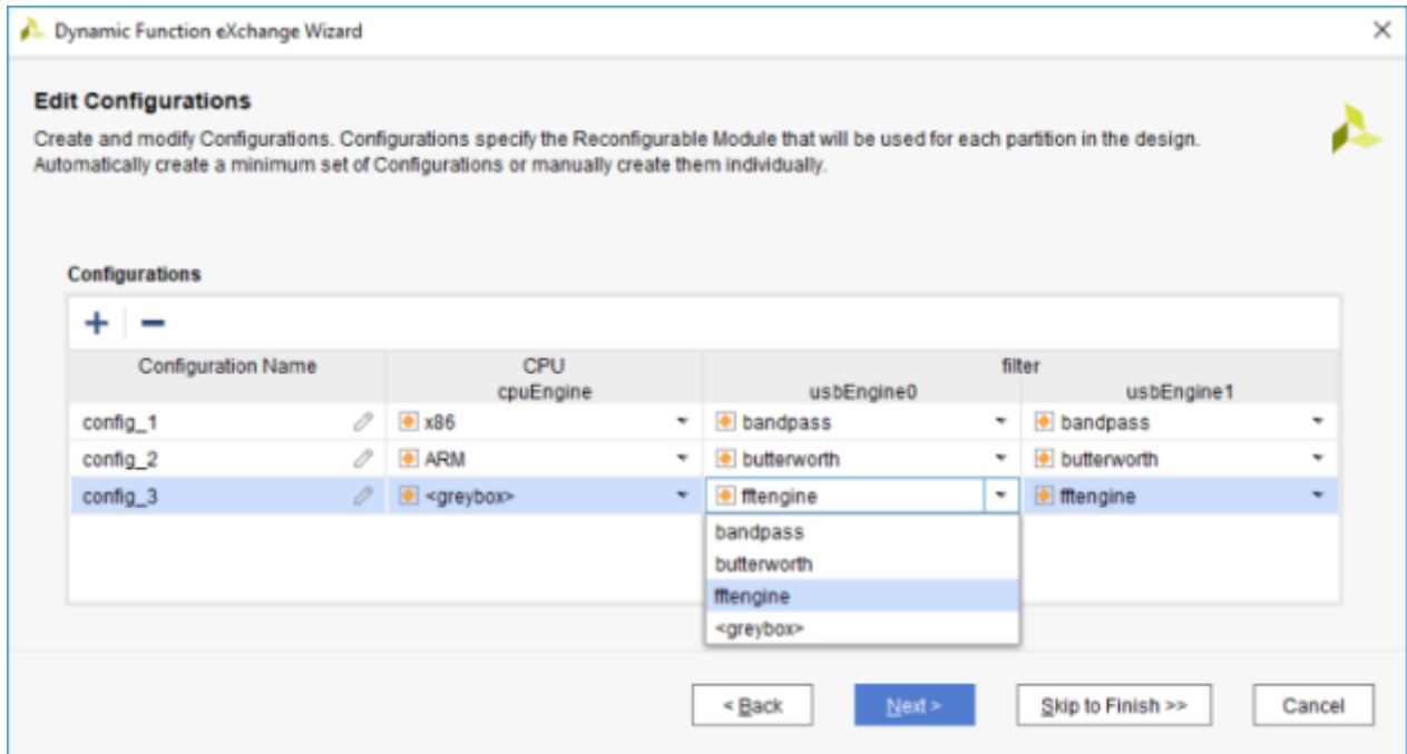
Figure 30: Edit Configurations after automatic generation of Configurations
