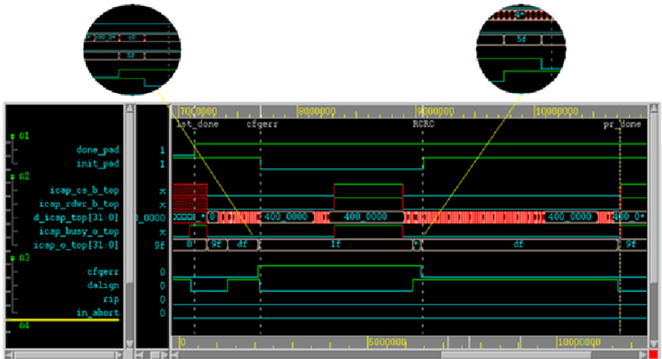
Figure 63: Vivado Logic Analyzer Display for Dynamic Function eXchange
