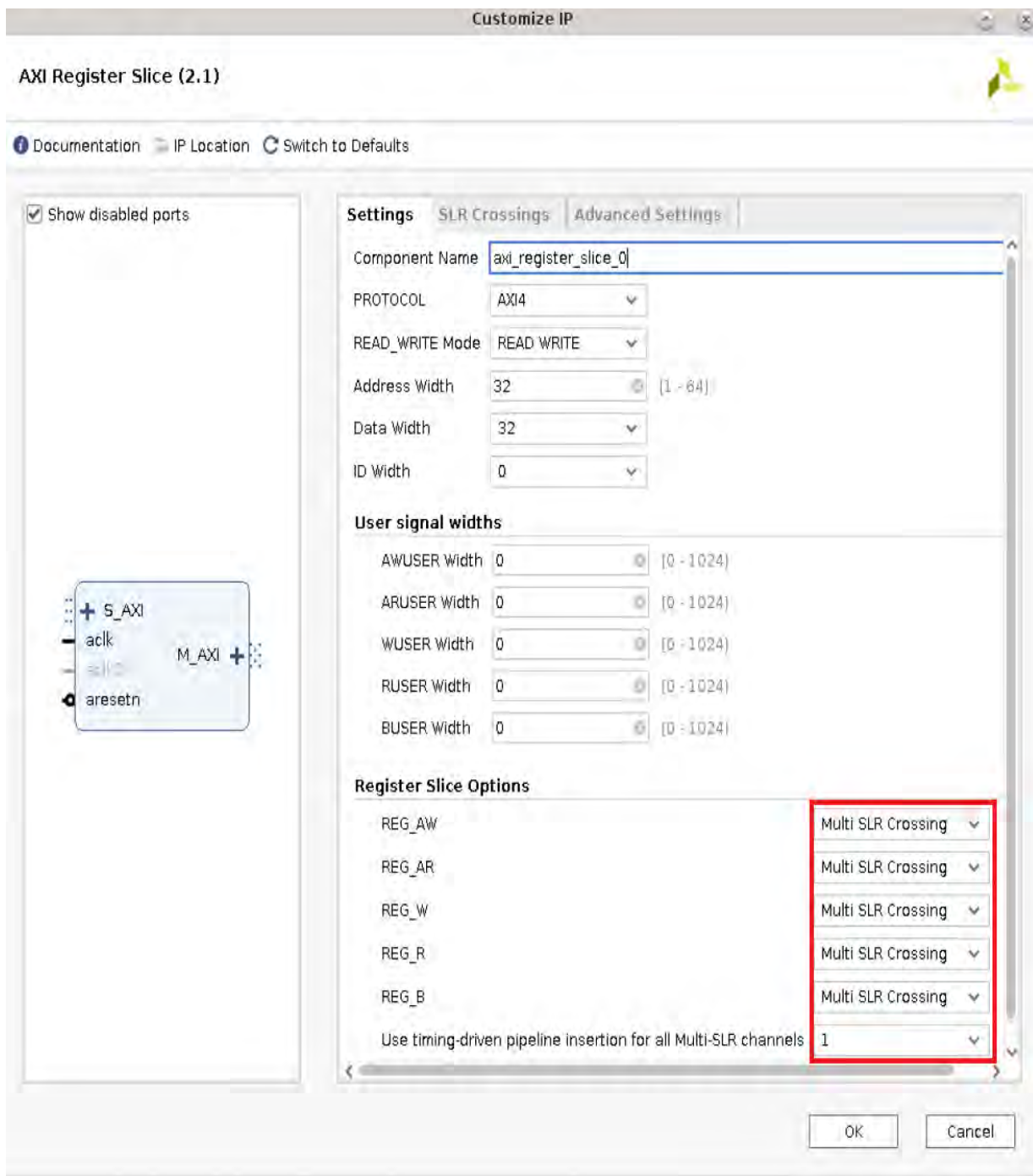
Figure 2-18: Example AXI Register Slice IP Settings to Enable Auto-Pipelining Feature
