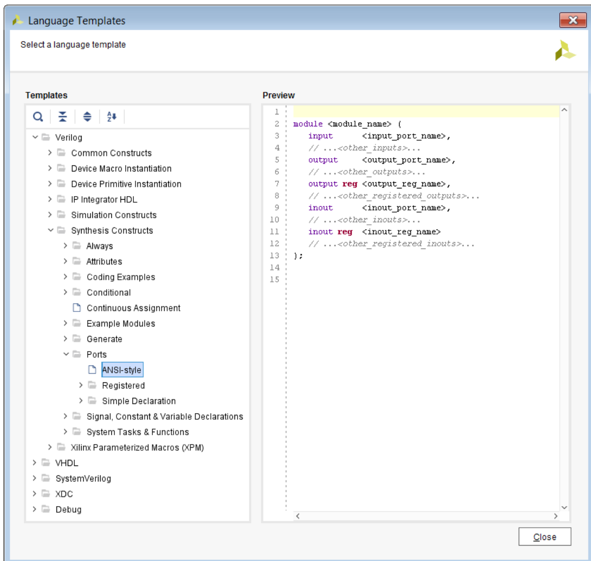
Figure 9: Language Templates
