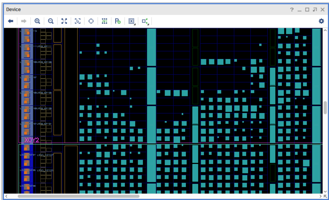
Figure 49: Device Window
