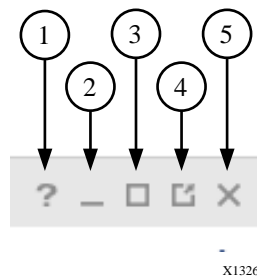
Figure 25: Window Controls
