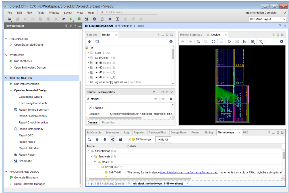
Figure 10: Implemented Design
