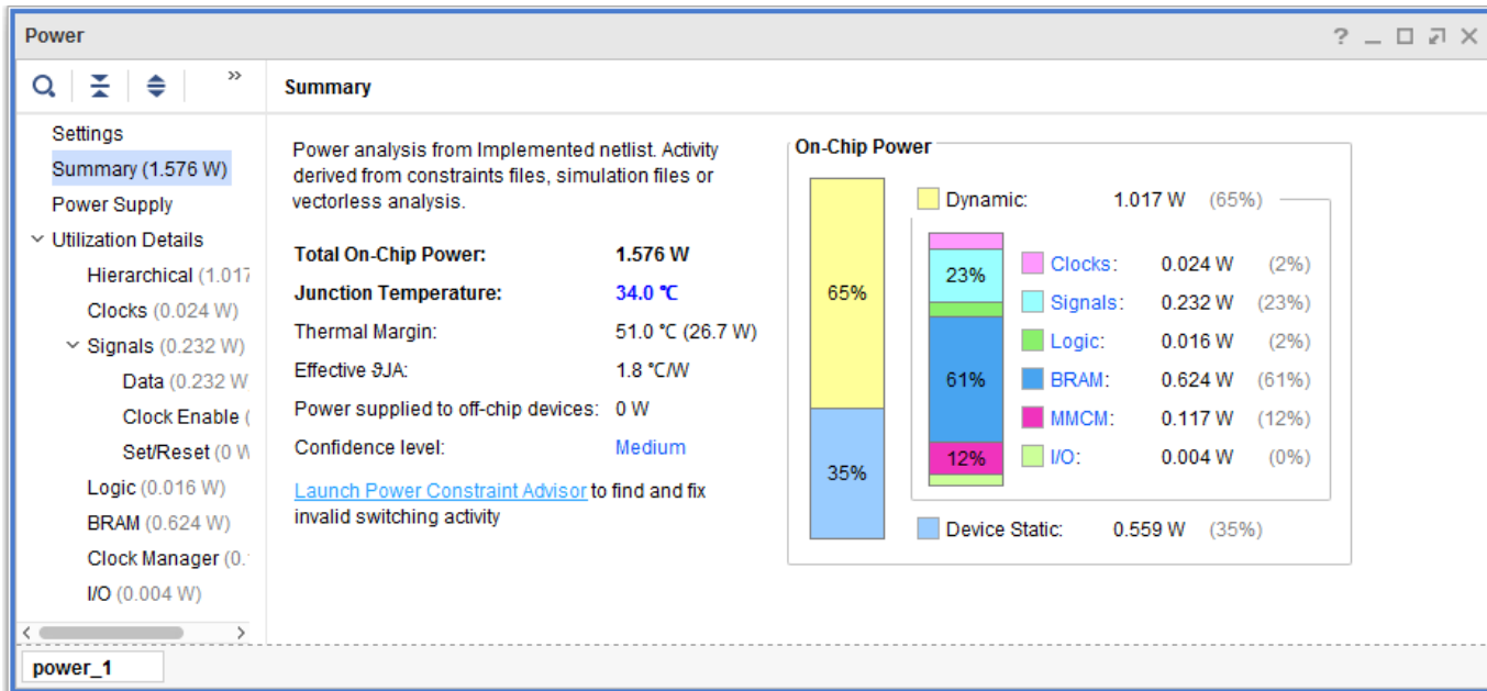
Figure 59: Power Report – Vectorless Analysis with Junction Temperature Supplied
