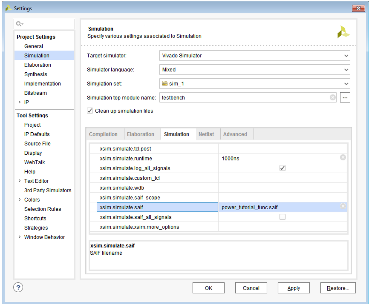
Figure 23: Simulation Settings – Entering SAIF File Setting
