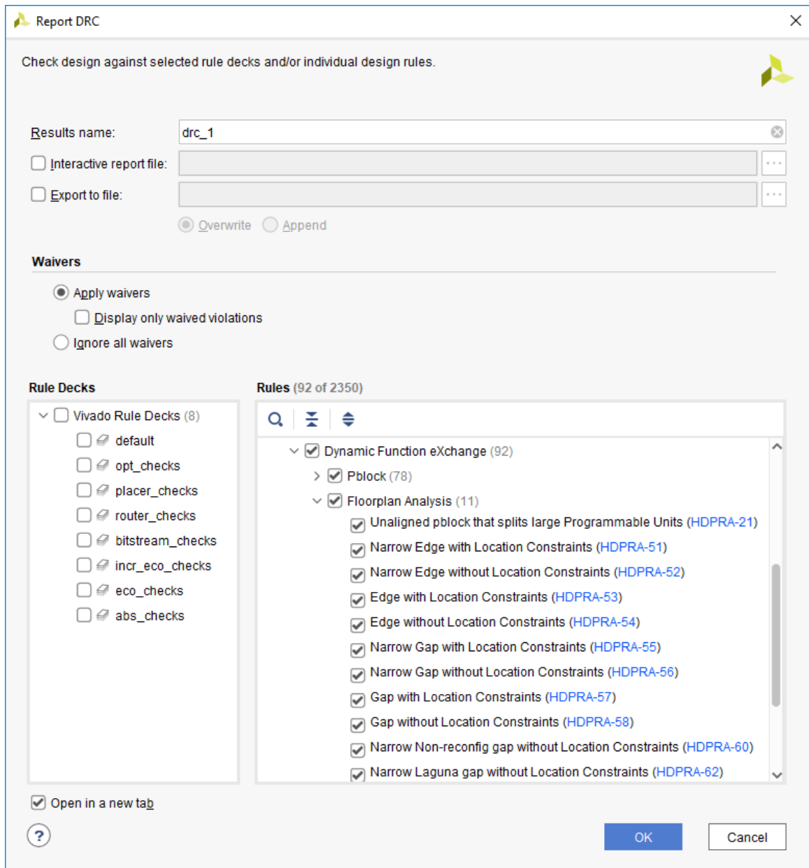
Figure 59: Checking Partial Reconfiguration DRCs
