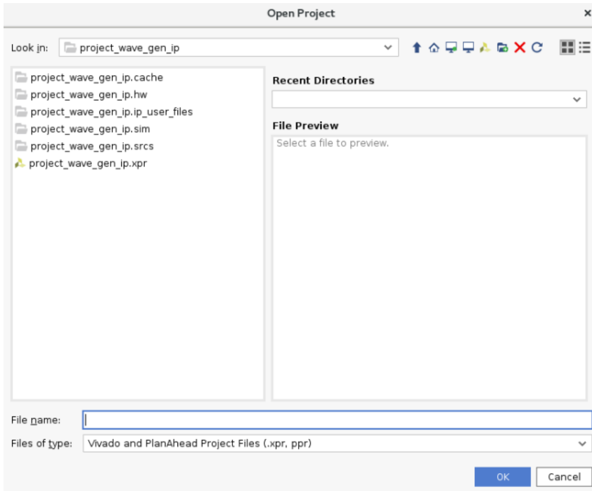
Figure 2: Open Project
