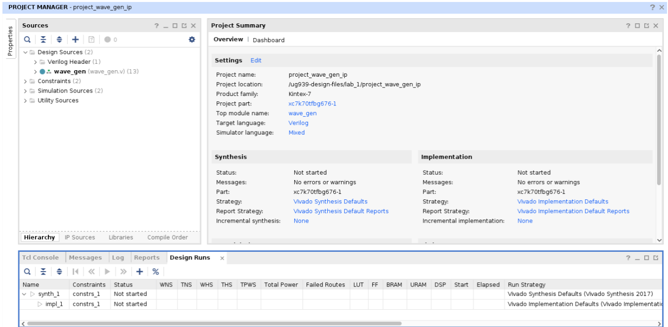
Figure 3: Default Layout
