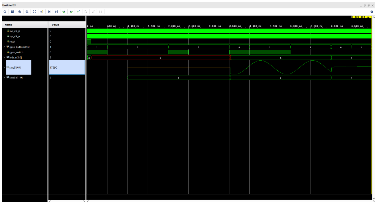
Figure 19: Design Bug - Wave View
