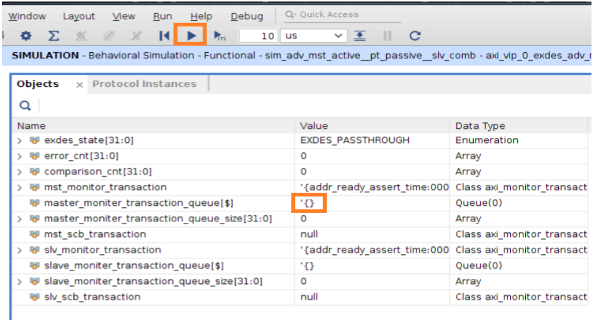
Figure 40: Objects Window
