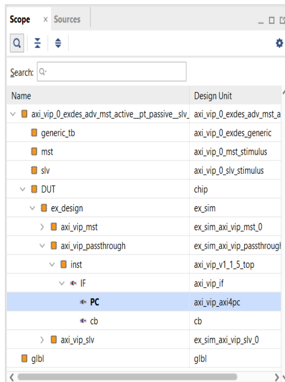
Figure 50: Scope Window
