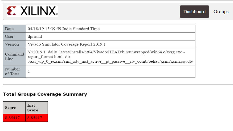
Figure 47: XCRG Dashboard
