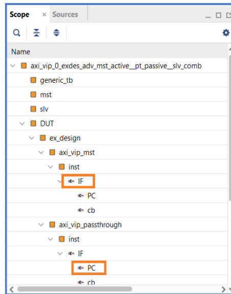
Figure 35: Scope Window
