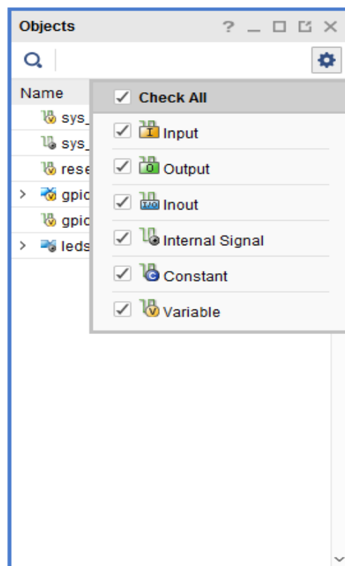
Figure 20: Object Filters
