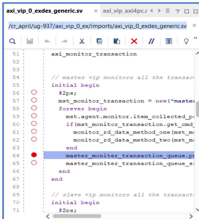
Figure 39: Text Editor
