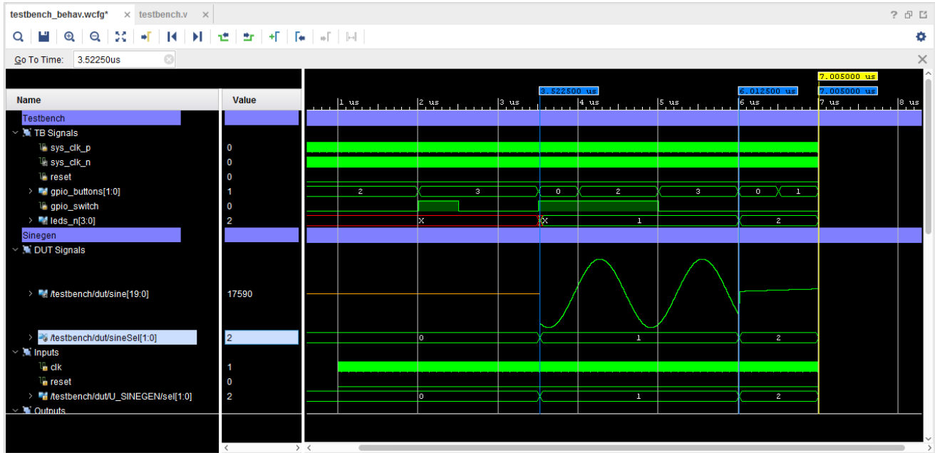
Figure 25: Using Markers
