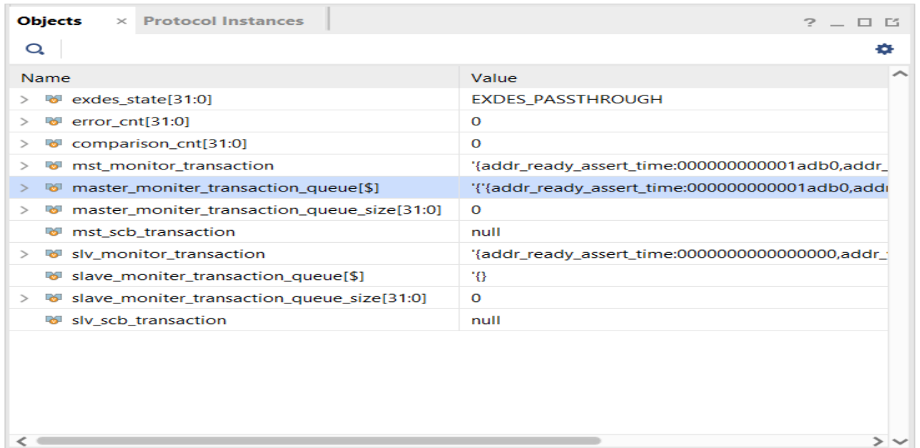
Figure 41: Objects Window
