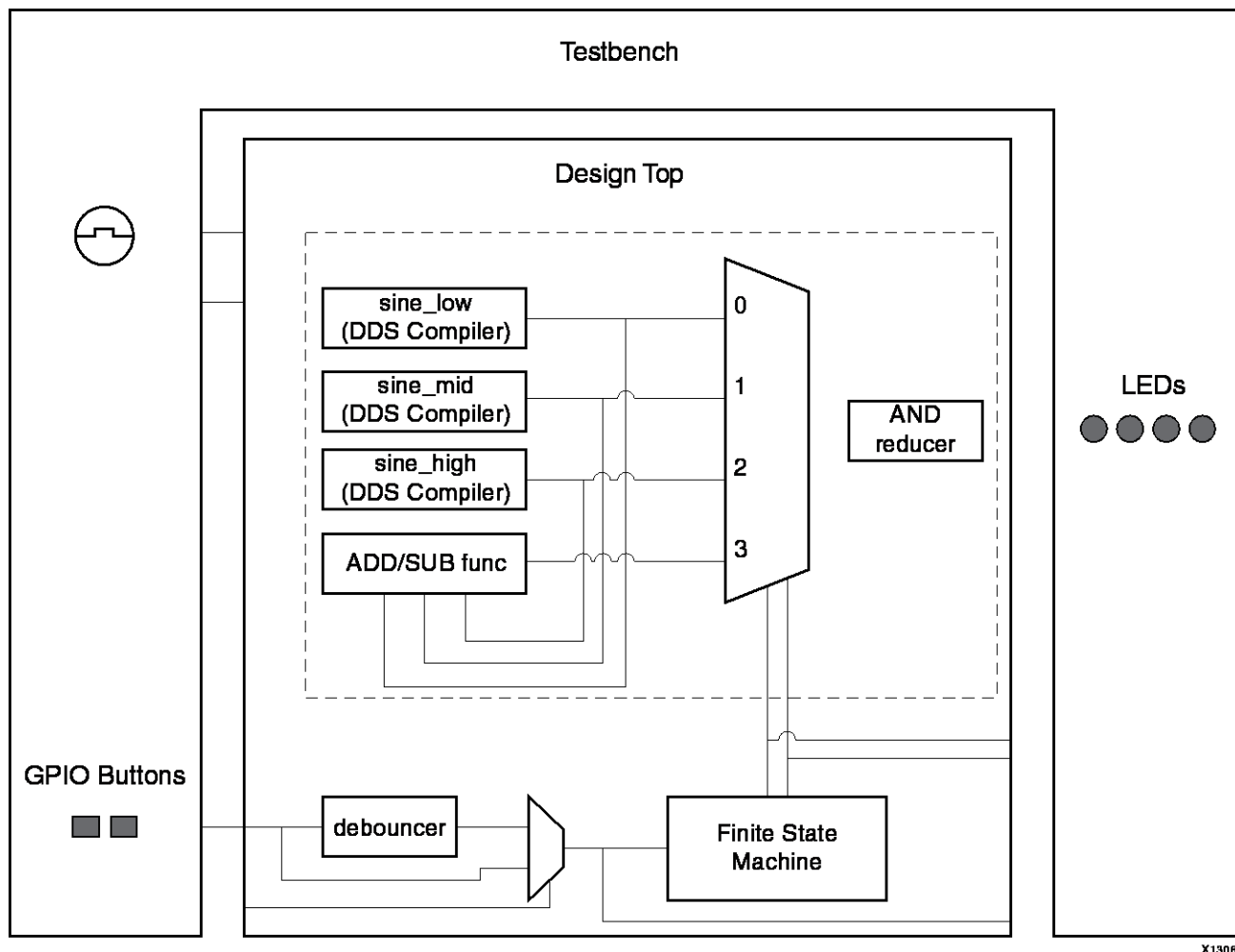
Figure 1: Tutorial Design
