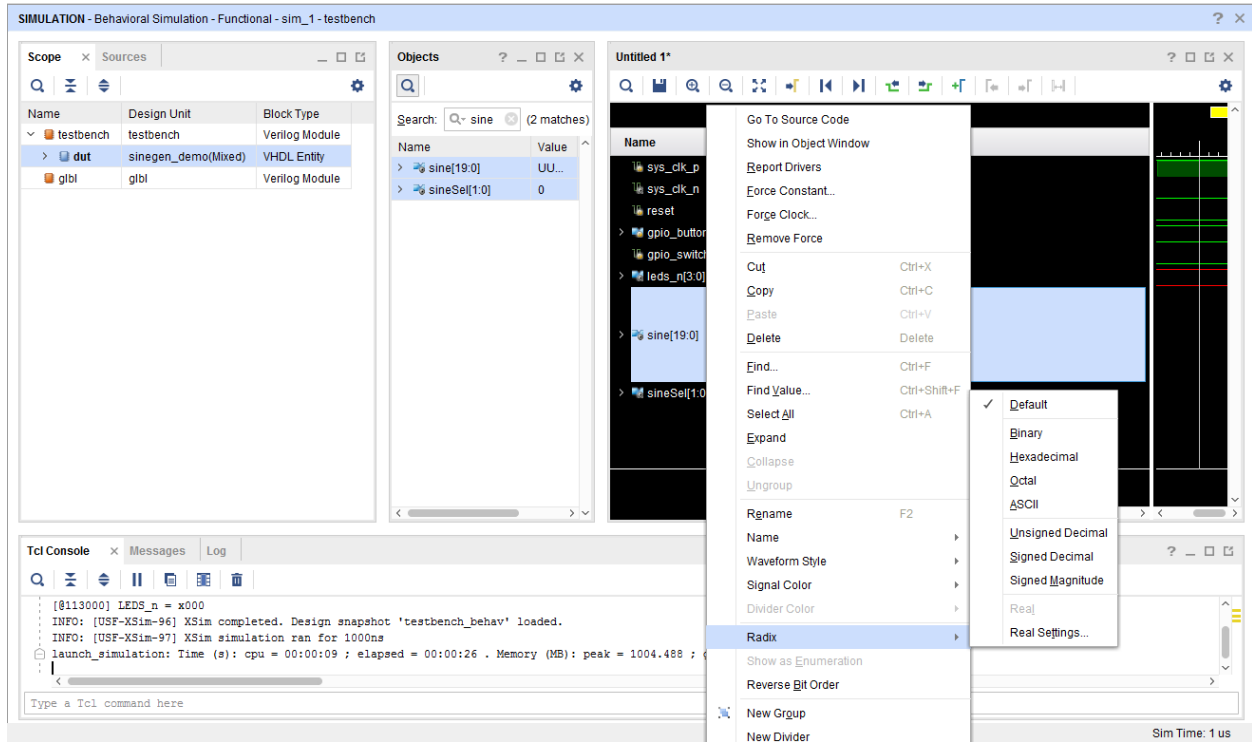
Figure 18: Enable Radix
