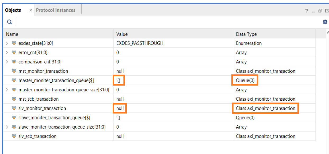
Figure 37: Objects Window
