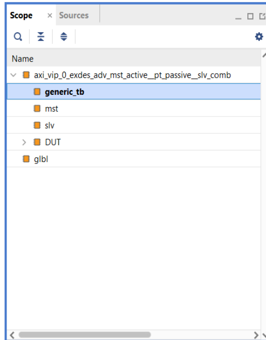
Figure 38: Scope Window
