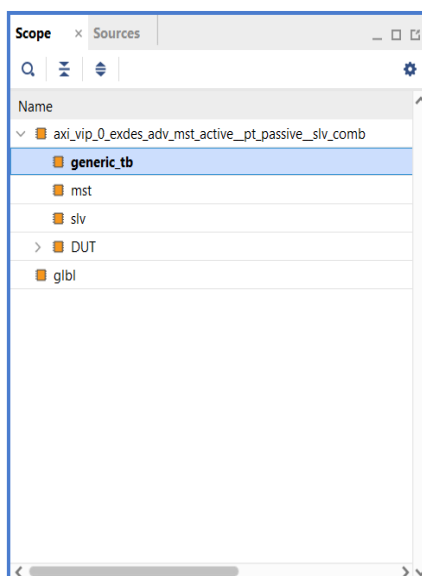
Figure 36: Scope Window
