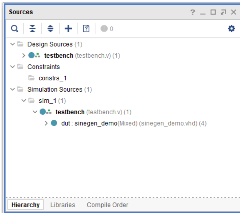
Figure 8: Sources window
