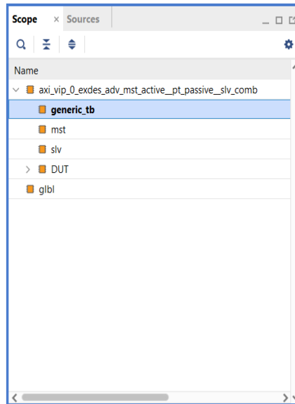
Figure 42: Scope Window
