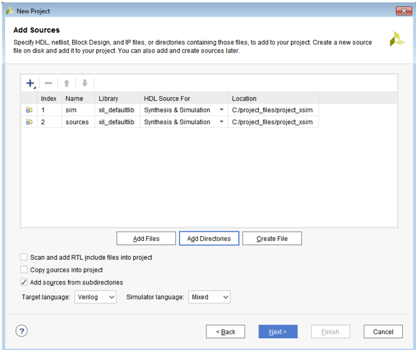
Figure 5: Add Sources
