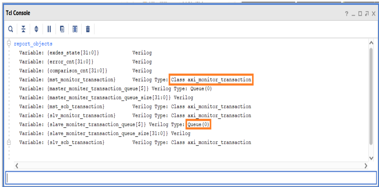
Figure 43: Tcl Console
