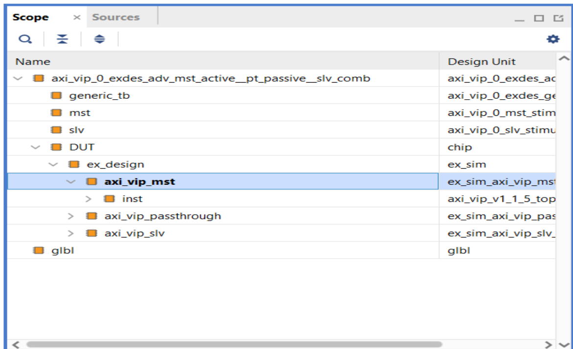
Figure 45: Scope Window
