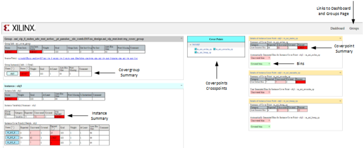
Figure 49: XCRG Detailed Report
