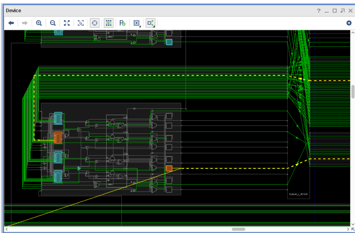
Figure 3-20: Assign Branching Route
