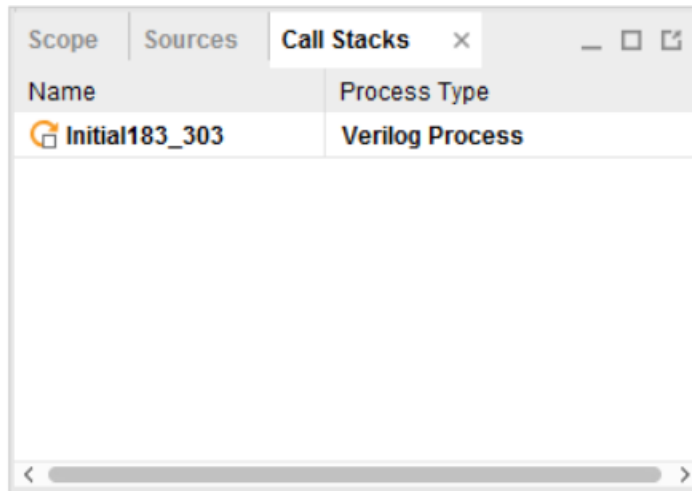
Figure 45: Call-Stack Window
