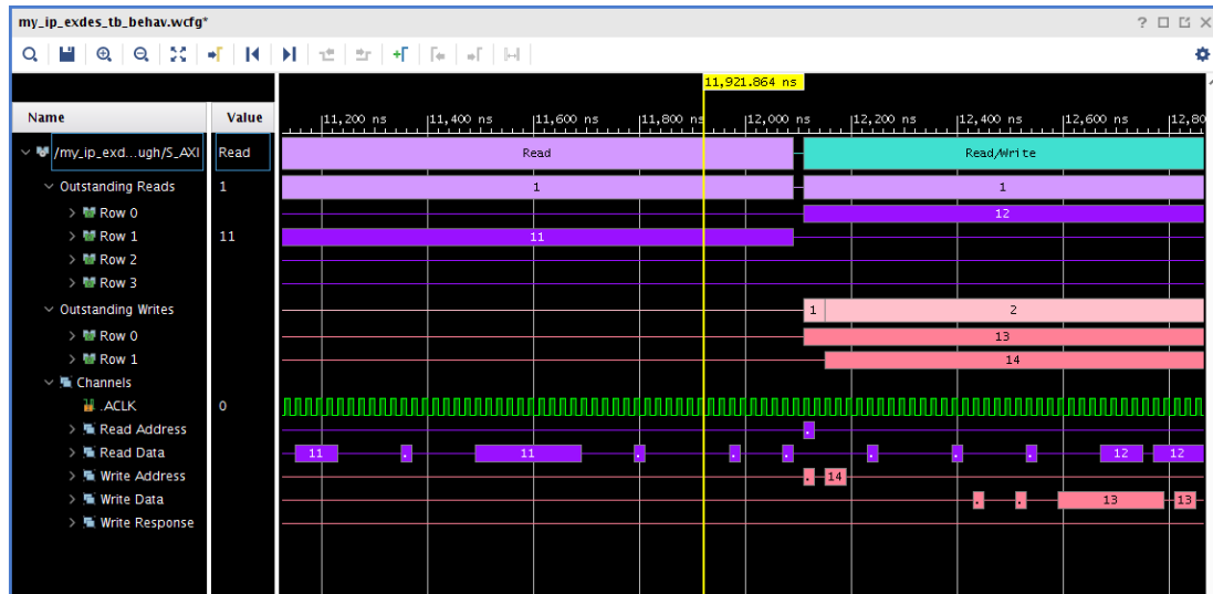
Figure 36: AXI-MM Interface
