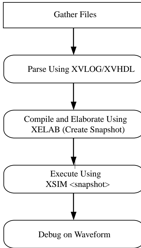
Figure 52: Behavioral Simulation Process
