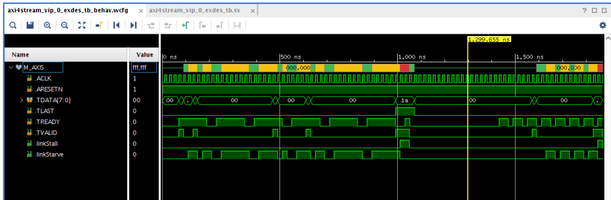
Figure 37: AXI-Stream (AXI-S) Interface
