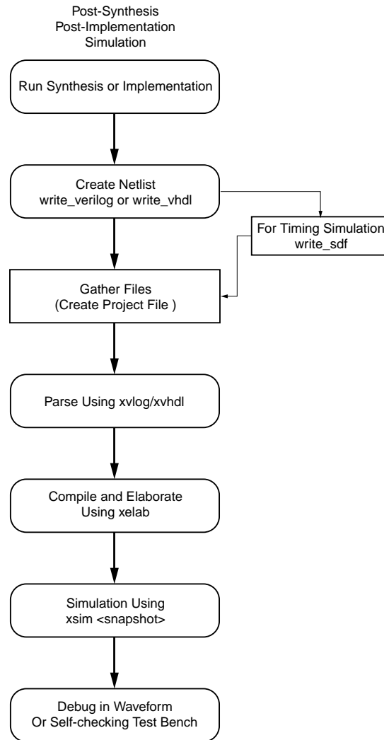
Figure 53: Post-Synthesis and Post-Implementation Simulation
