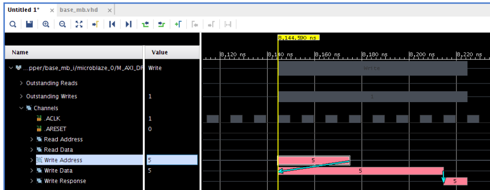
Figure 35: Transaction Bars with Associations
