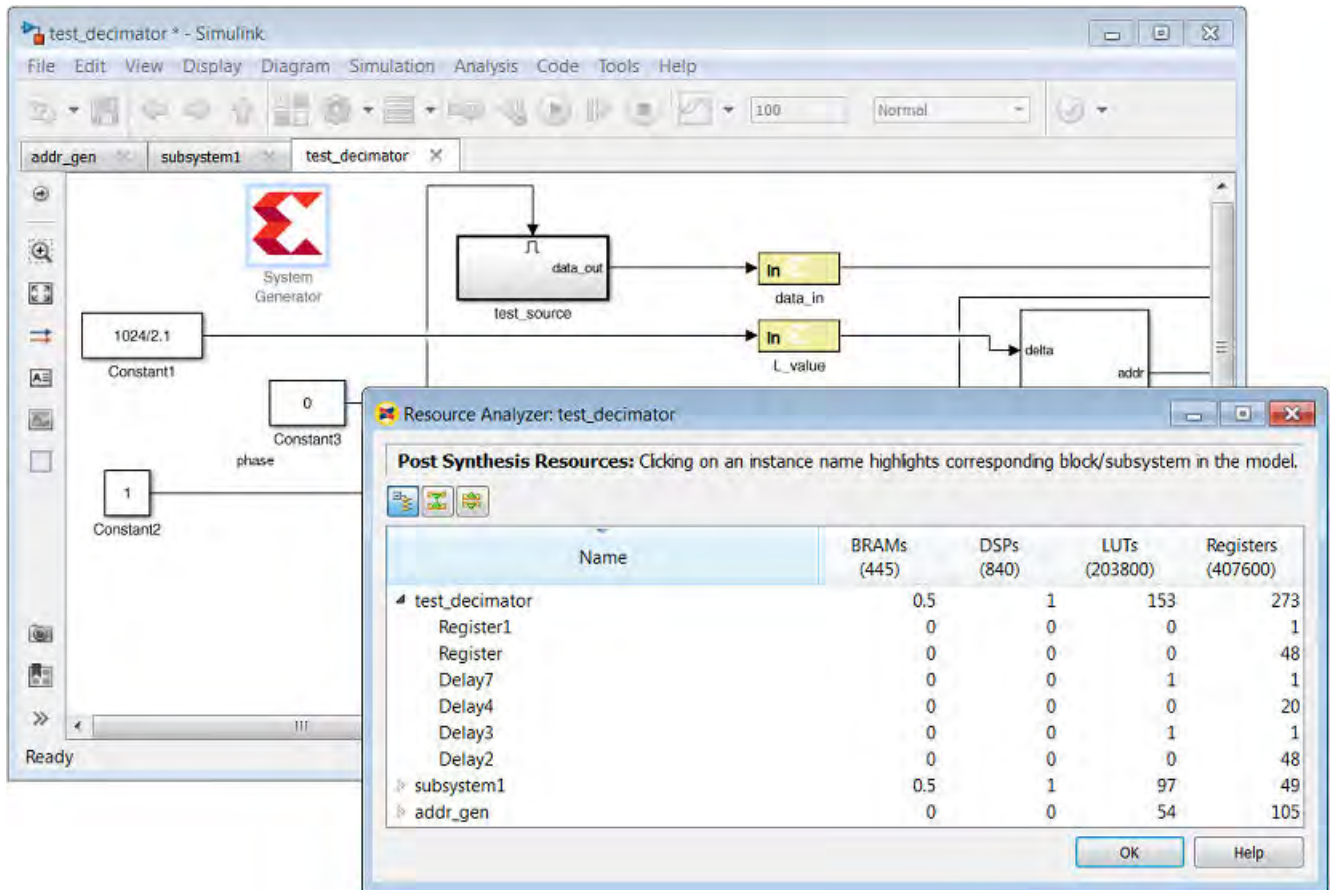
Figure 108: Resource Analyzer
