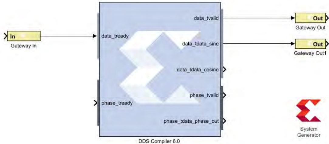
Figure 171: Model with Open Input and Output Ports
