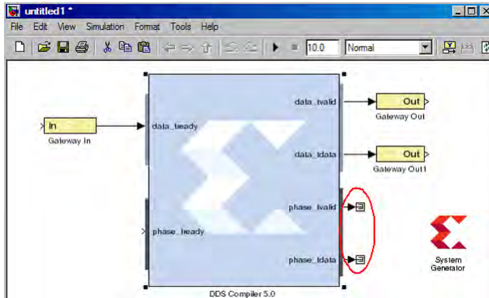
Figure 172: Terminated Output Ports
