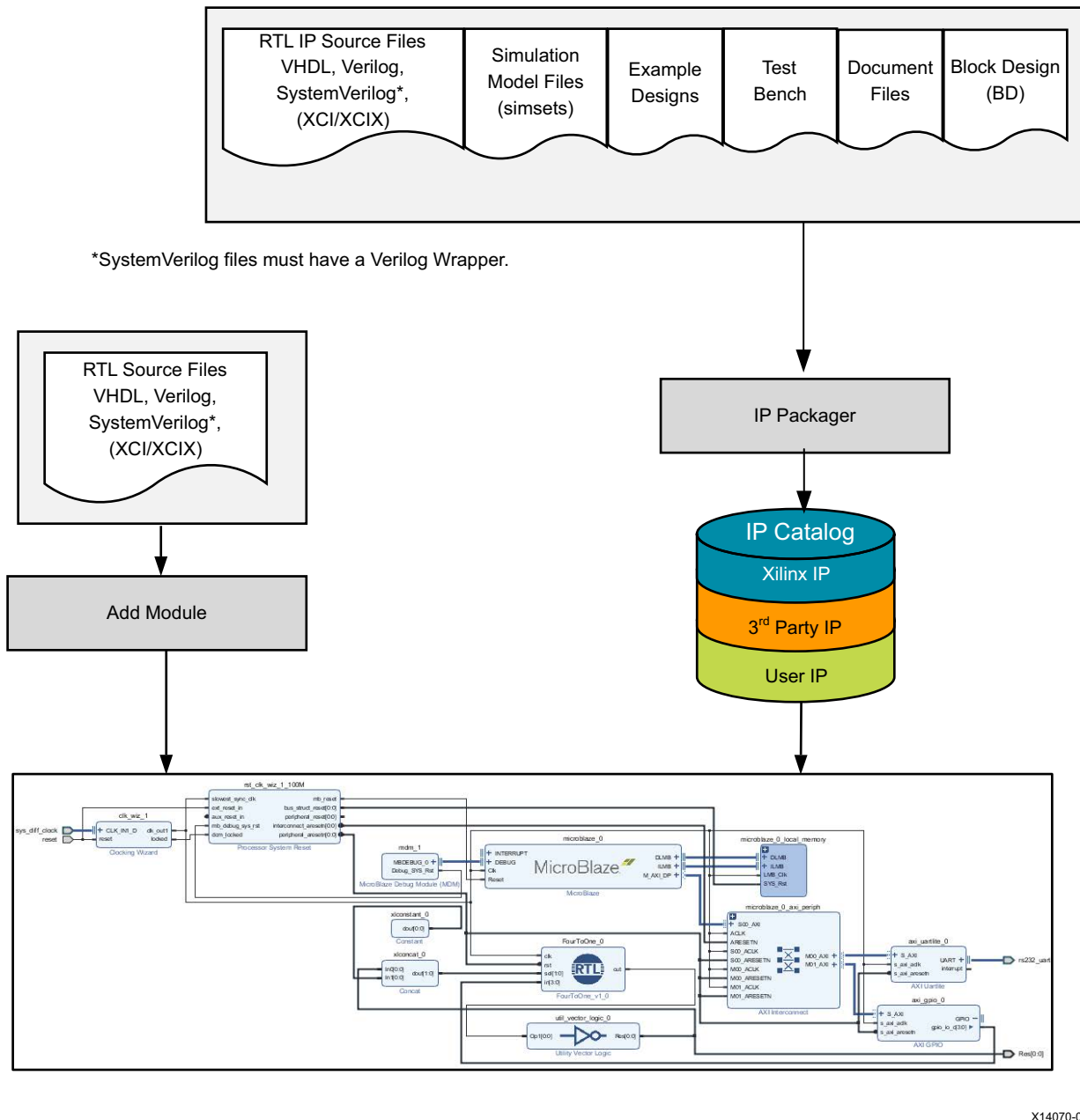
Figure 1-1: IP-Centric Design Flow
