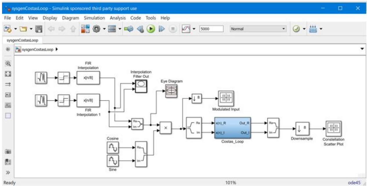
Figure 5: Hardware Co-Simulation
