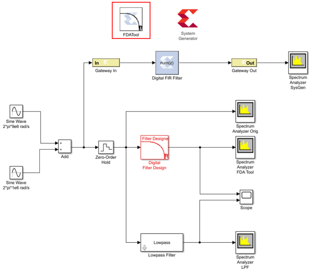
Figure 57: Spectrum Analyzer Block
