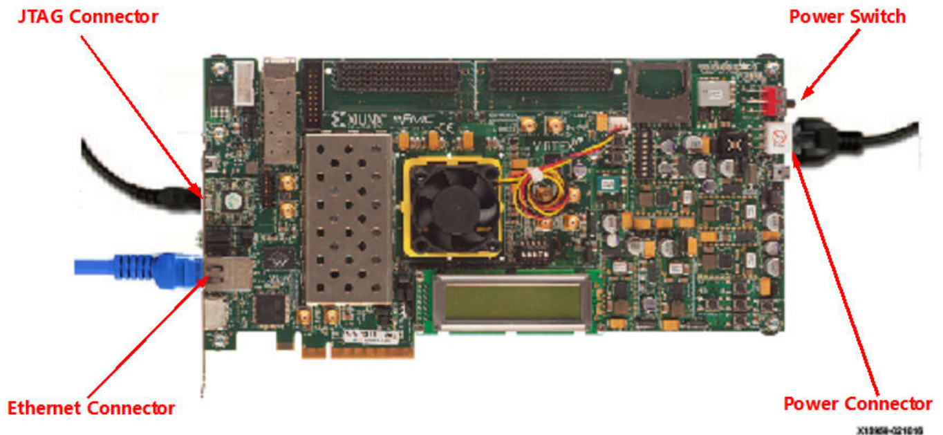
Figure 122: VC705 Board Ethernet Connections
