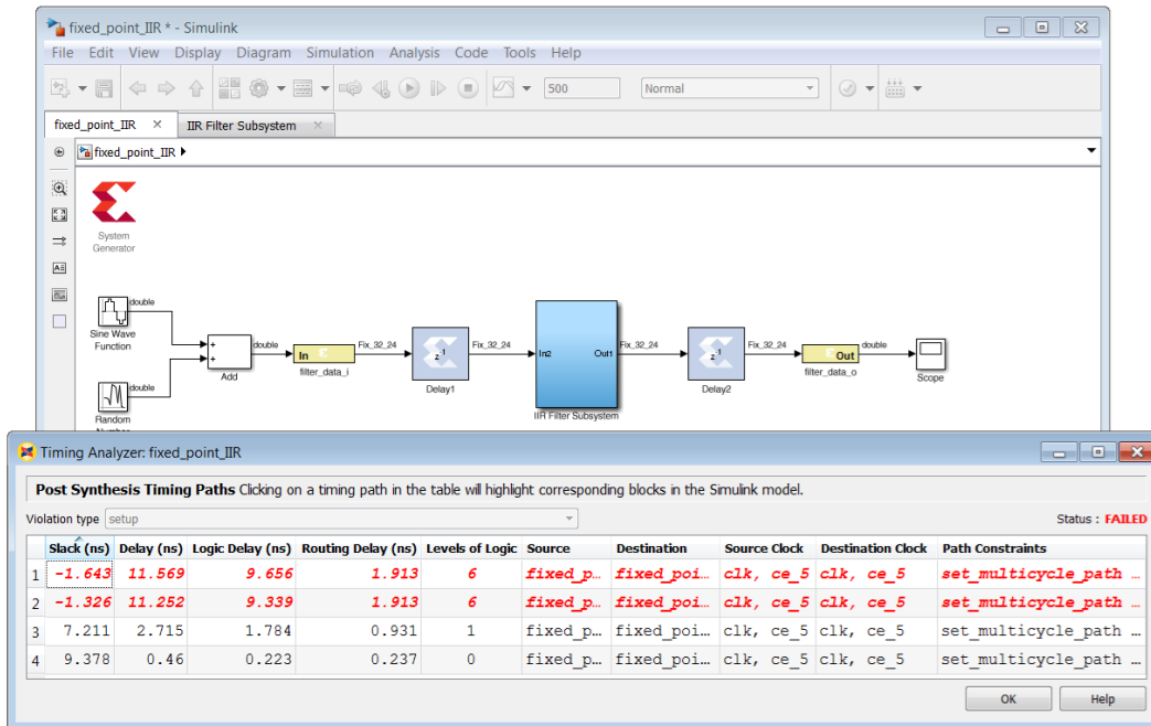
Figure 99: Timing Analyzer Table
