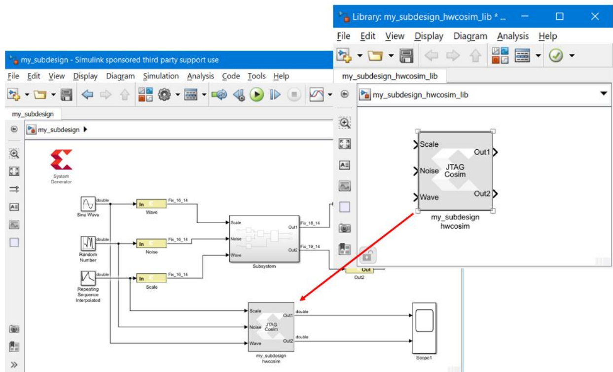
Figure 123: Hardware Co-Simulation Blocks
