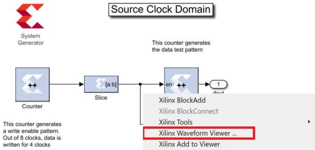
Figure 69: Source Clock Domain
