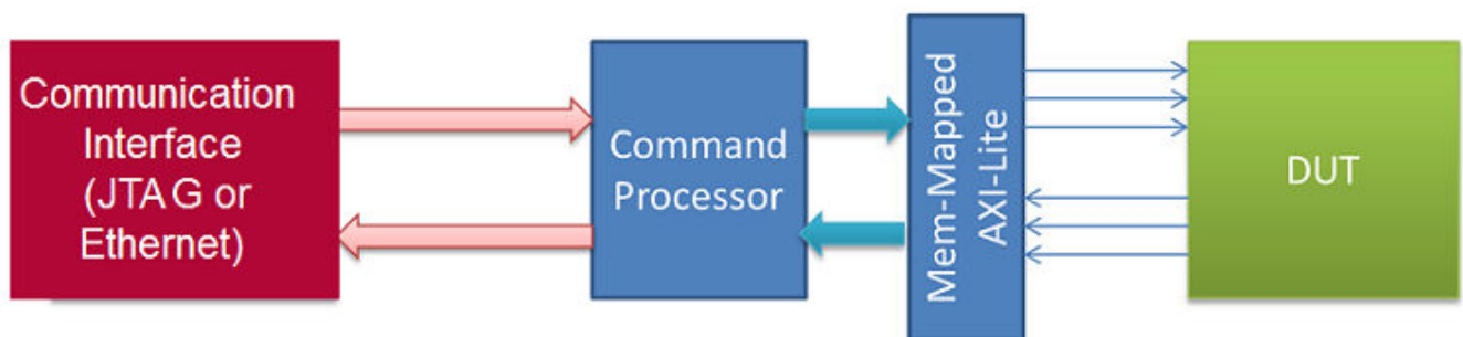
Figure 135: Hardware Co-Simulation Flow
