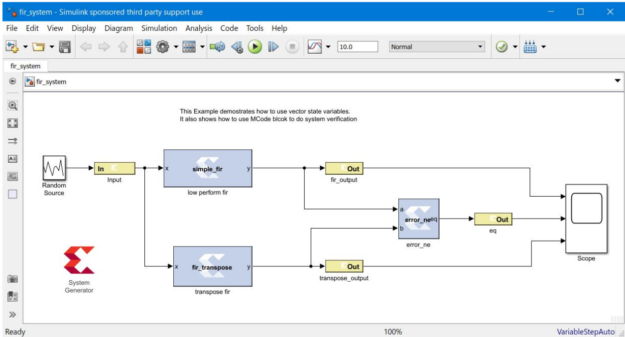
Figure 39: FIR Example
