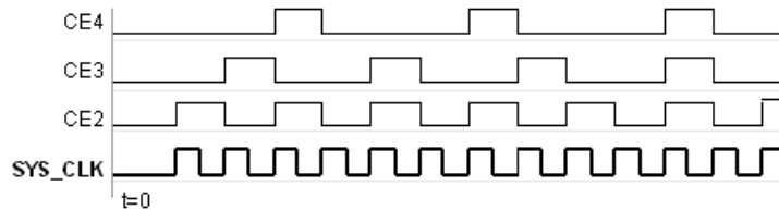
Figure 17: Timing Diagram
