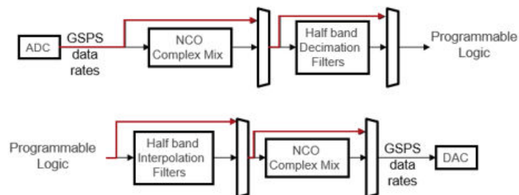
Figure 94: RFSoc Device
