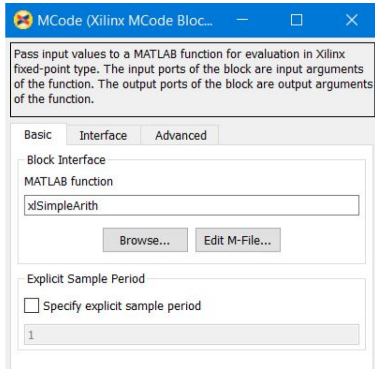
Figure 26: xISimpleArith Design
