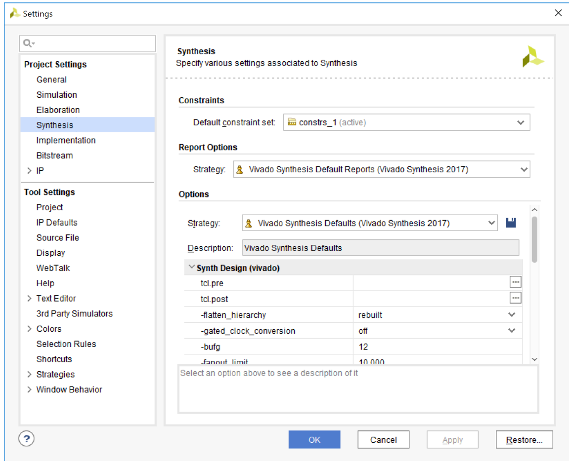
Figure 2-18: Synthesis Settings
