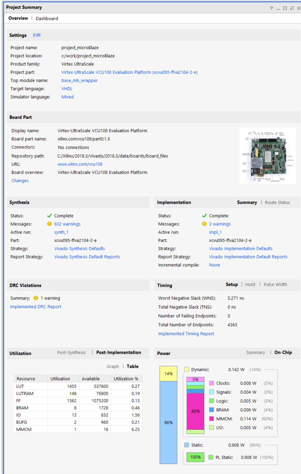
Figure 2-14: Project Summary
