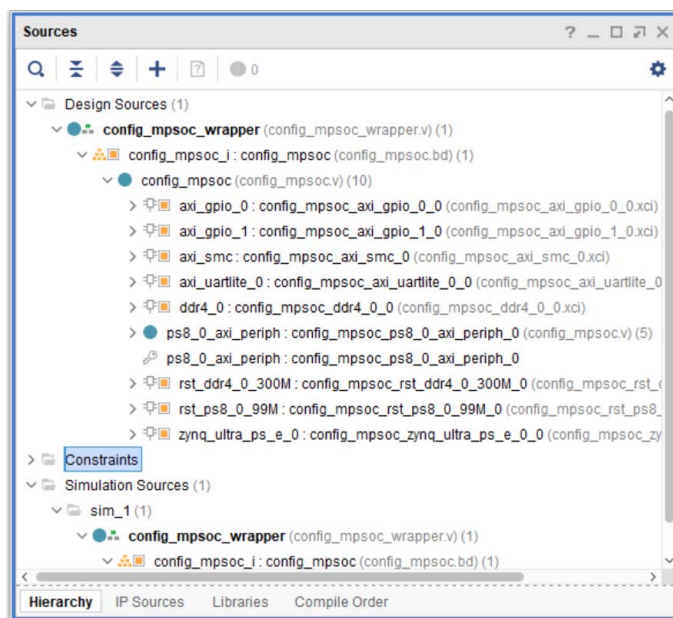
Figure 3-1: Sources Window
