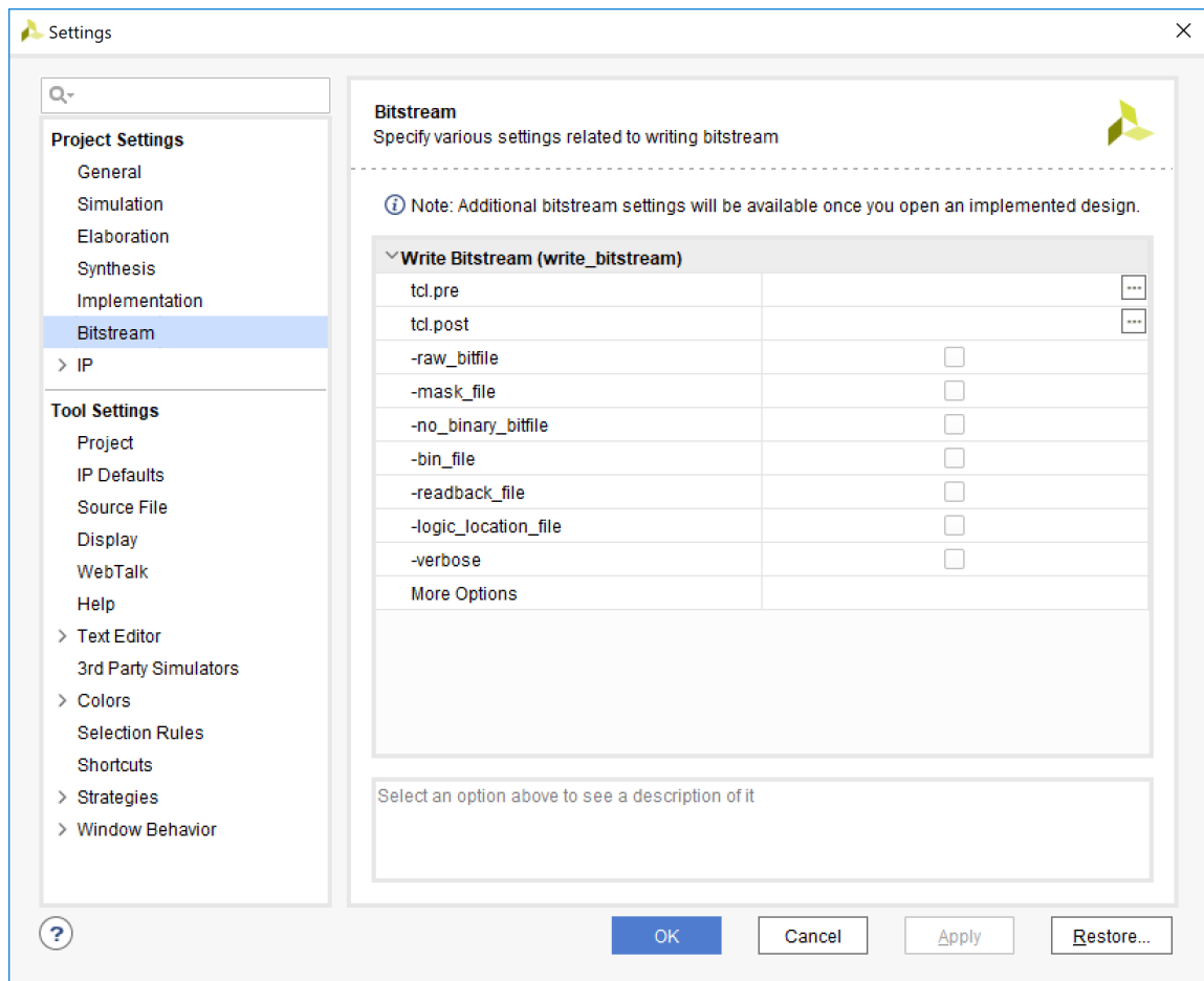
Figure 2-20: Bitstream Settings
