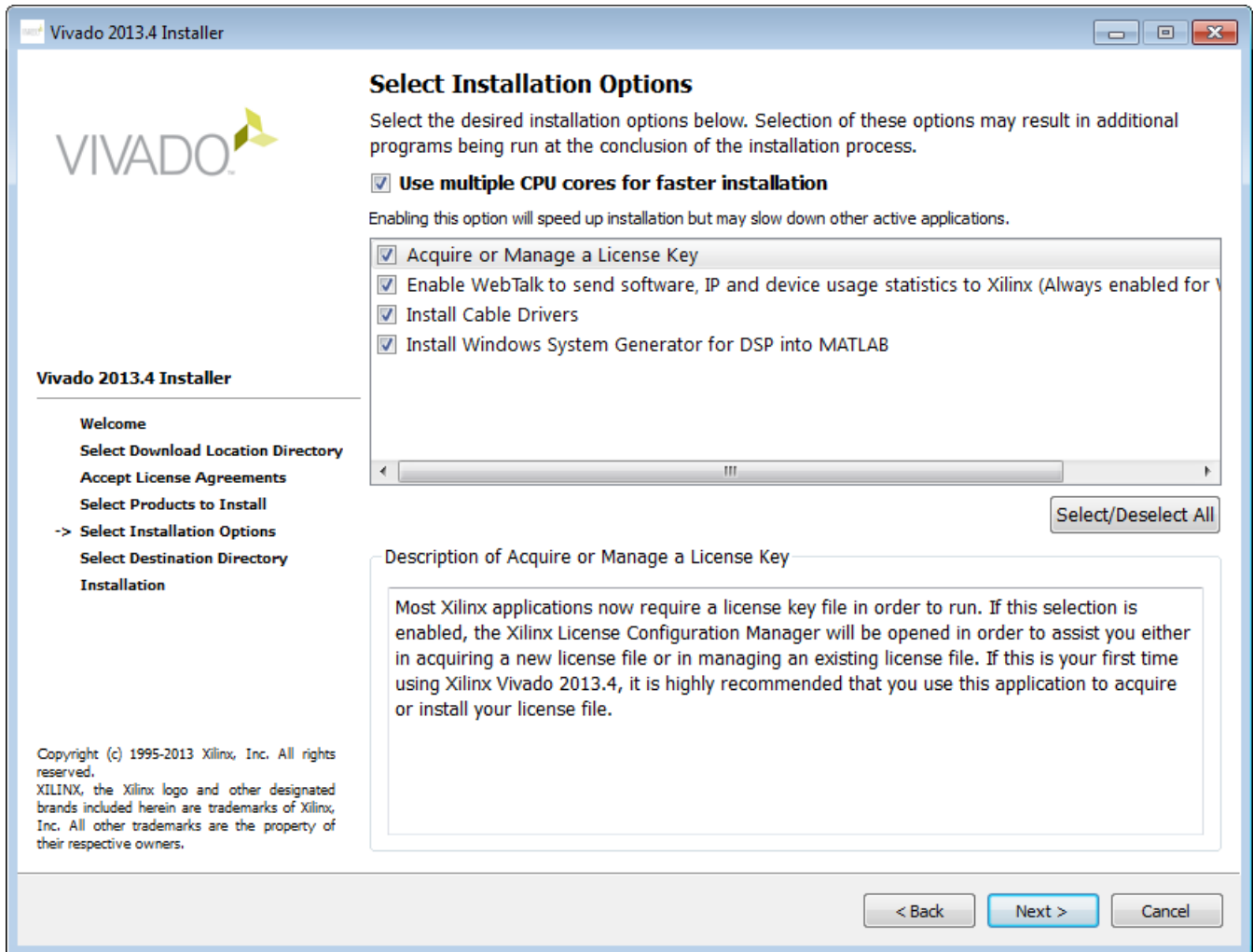
Figure 3-3: Vivado Design Suite Installation - Select Installation Options
