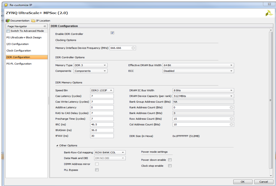
Figure 4-7: DDR Controller Options
