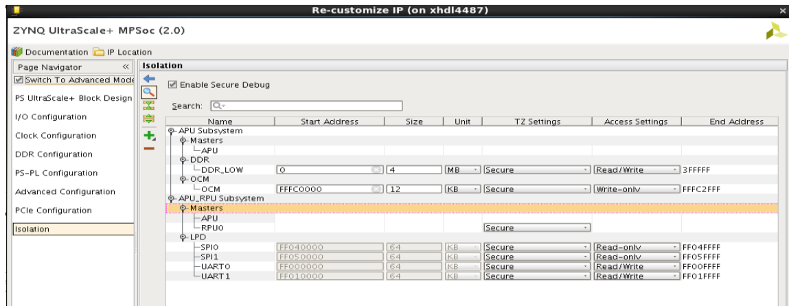
Figure 4-23: Isolation Configuration -- Masters List
