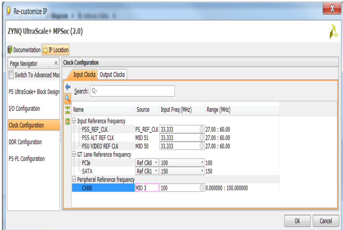
Figure 4-3: Clock Configuration Page (Input Clocks)
