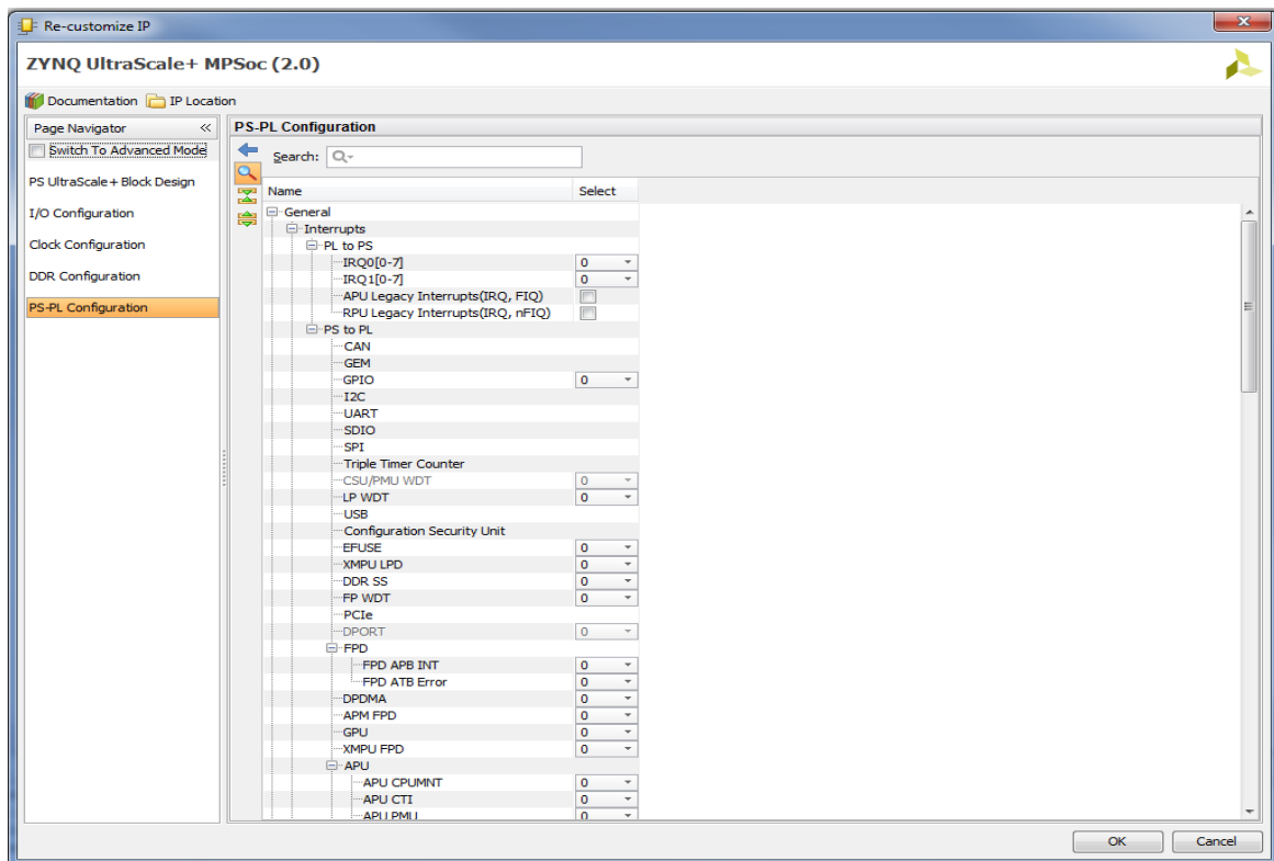
Figure 4-8: PS-PL Configuration Page
