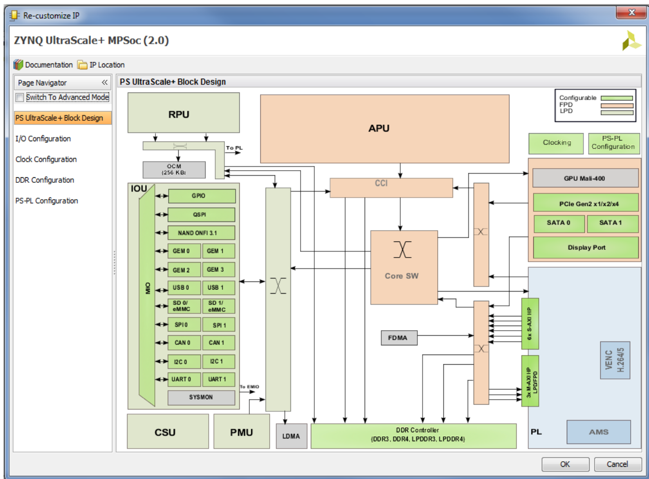
Figure 4-1: PS Zynq UltraScale+ Block Design Page
