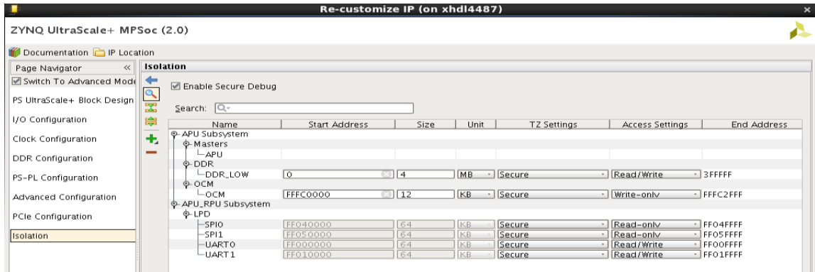
Figure 4-20: Access Settings as Read-Only
