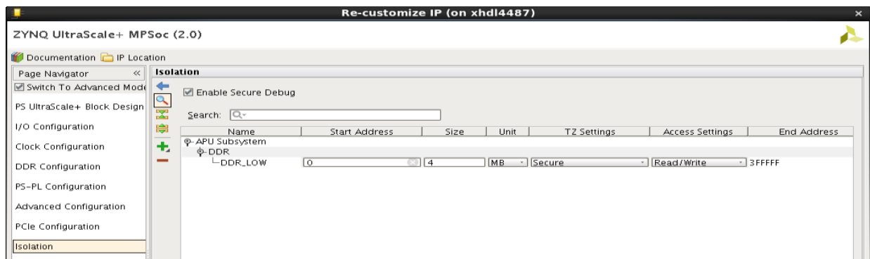
Figure 4-15: Setting TZ as Secure from the TZ Settings
