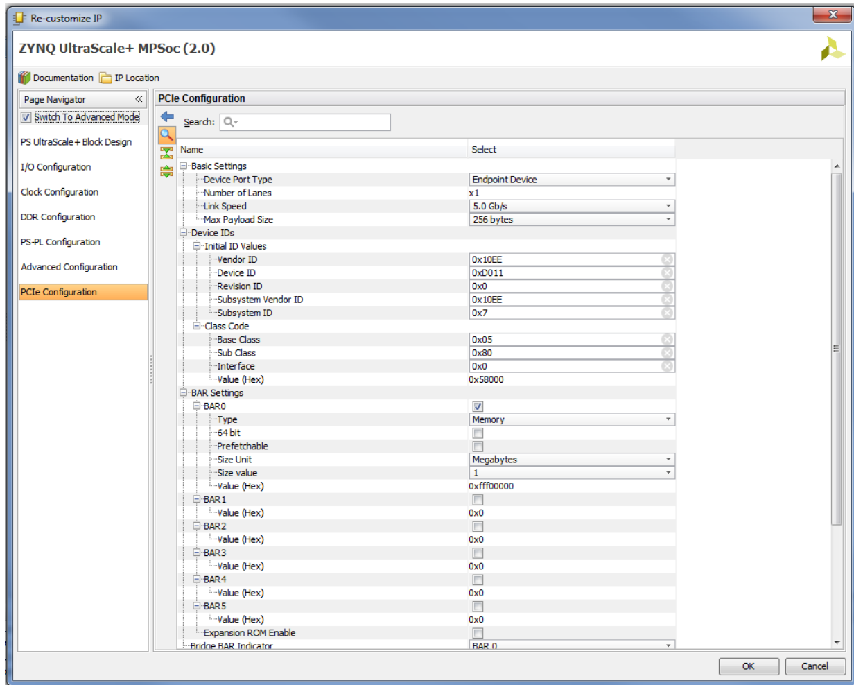
Figure 4-10: PCIe Configuration
