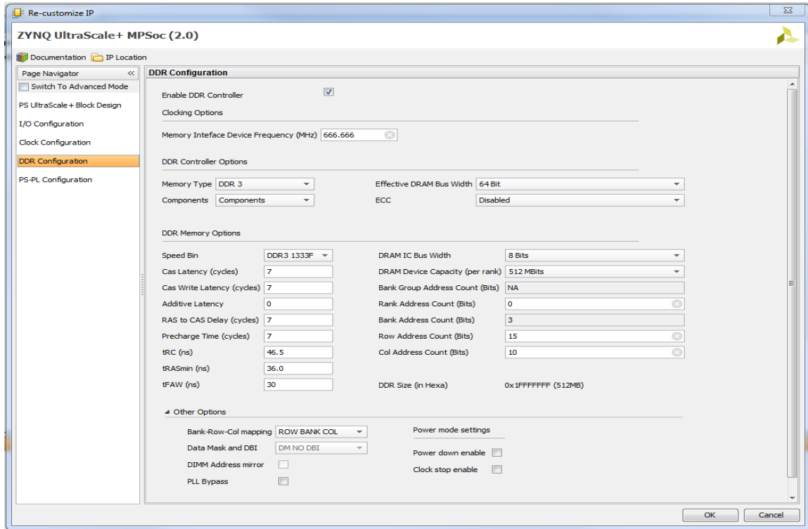
Figure 5-1: DDR Configuration
