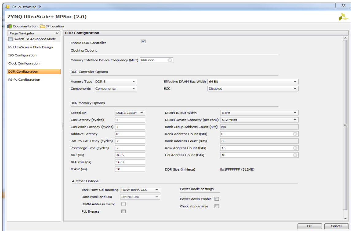
Figure 5-7: DDR Configuration
