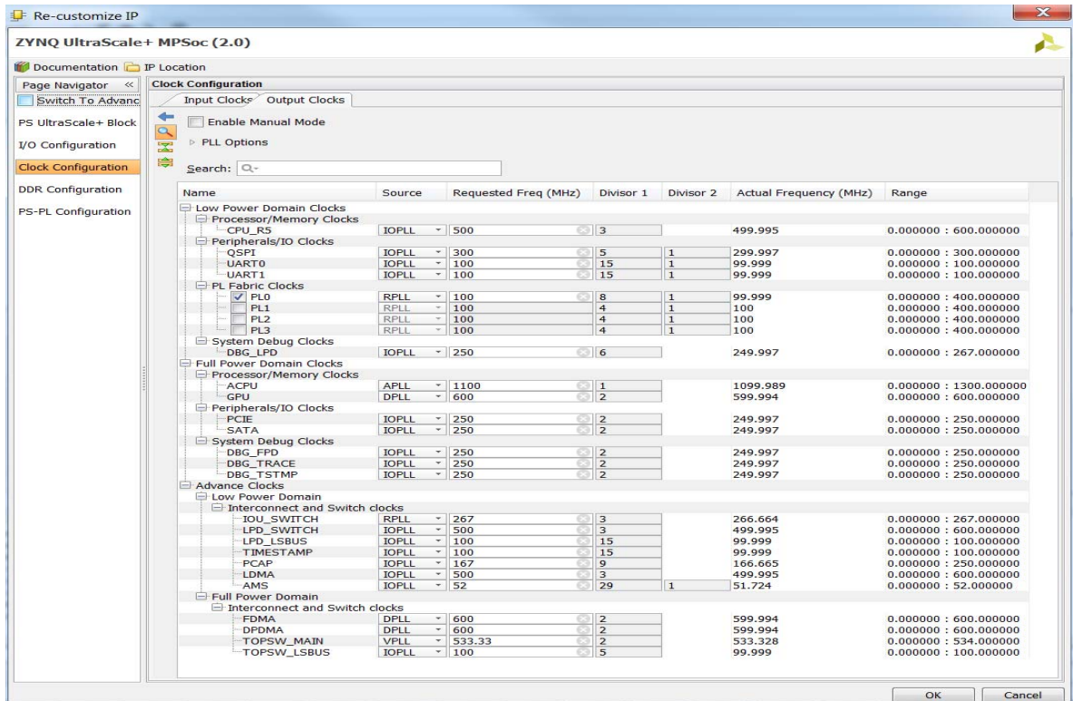
Figure 4-4: Clock Configuration Page (Output Clocks)
