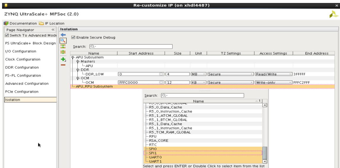
Figure 4-19: Selecting LPD
