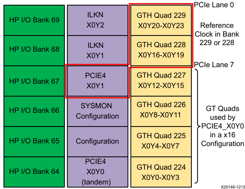
Figure B-3: Alternative PCIe GT Location Selection
