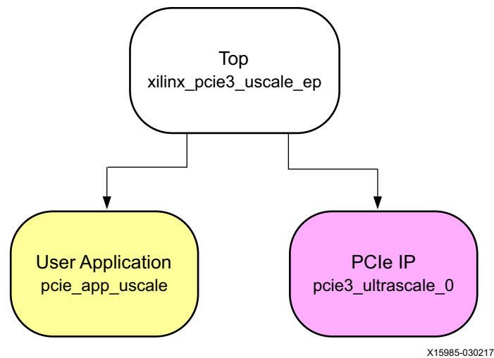
Figure 3-13: Required Design Hierarchy for Tandem With Field Updates
