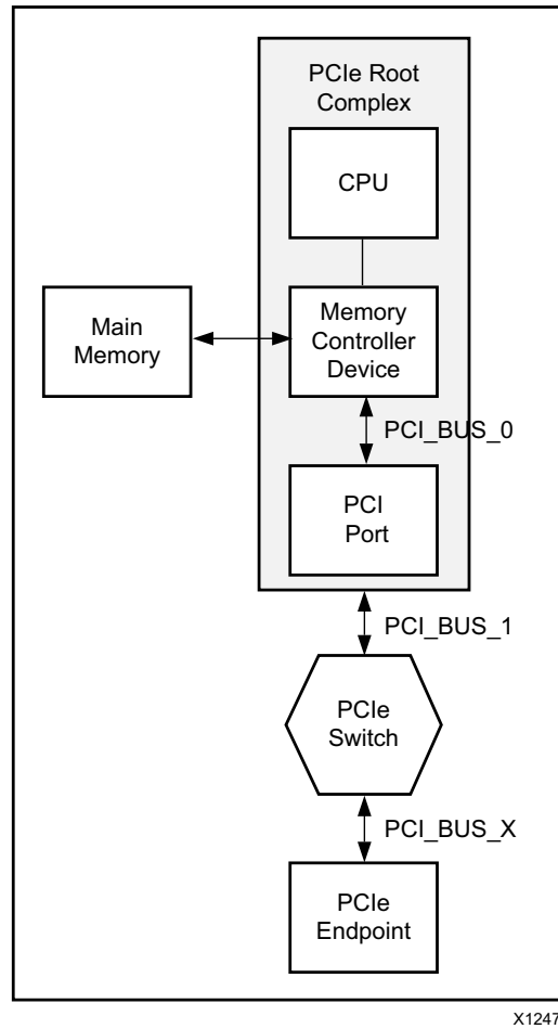
Figure 5-3: System Overview
