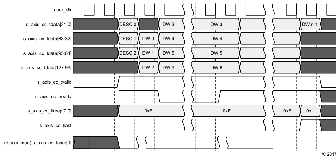
Figure 3-38: Transfer of a Normal Completion on the Completer Completion Interface (Address-Aligned Mode, 128-Bit Interface)
