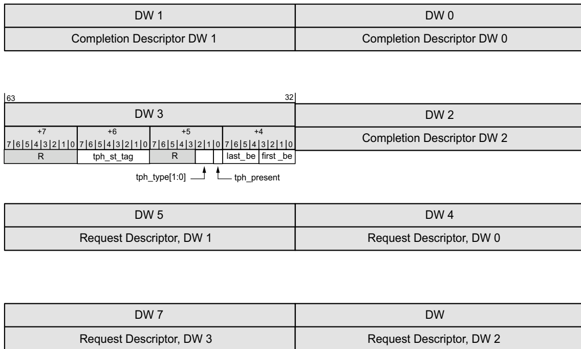
Figure 3-40: Composition of the AXI4-Stream Packet for UR and CA Completions
