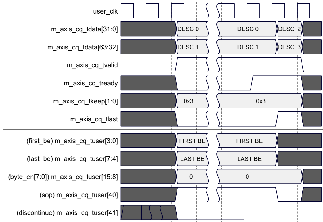
Figure 3-29: Memory Read Transaction on the Completer Request Interface (64-Bit Interface)
