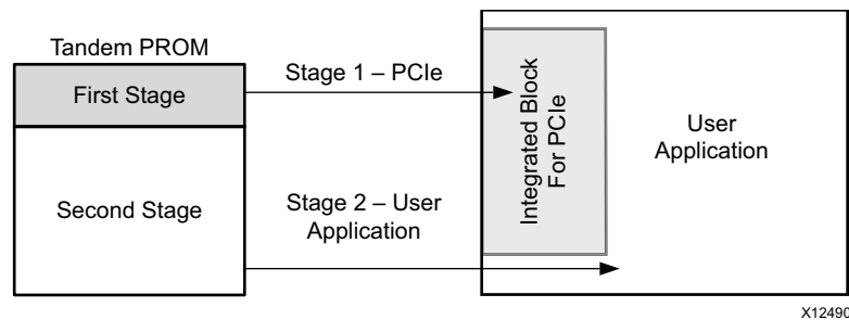
Figure 3-5: Tandem PROM Bitstream Load Steps
