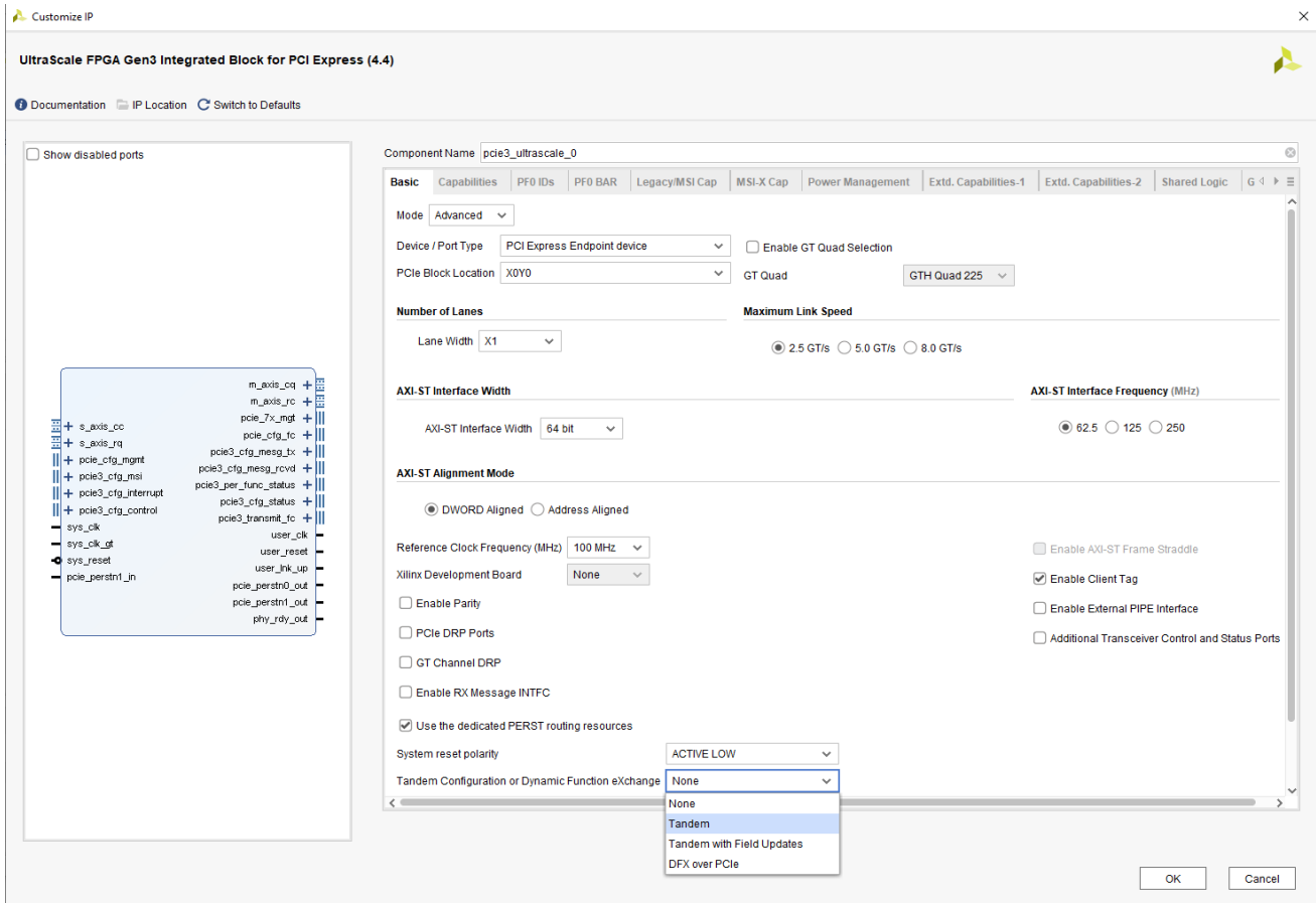
Figure 3-10: Tandem PCIe
