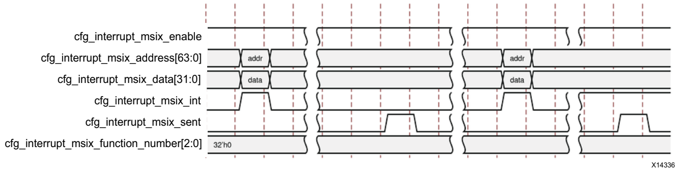
Figure 3-74: MSI-X Mode
