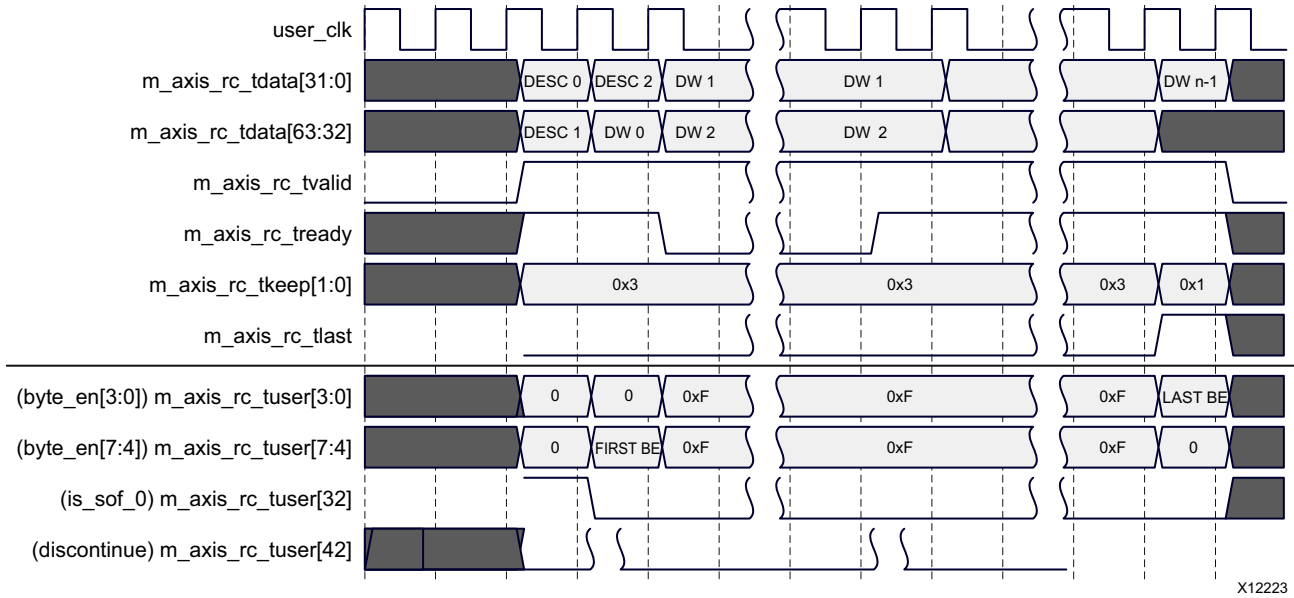
Figure 3-64: Transfer of a Completion with Data on the Requester Completion Interface (Dword-Aligned Mode, 64-Bit Interface)
