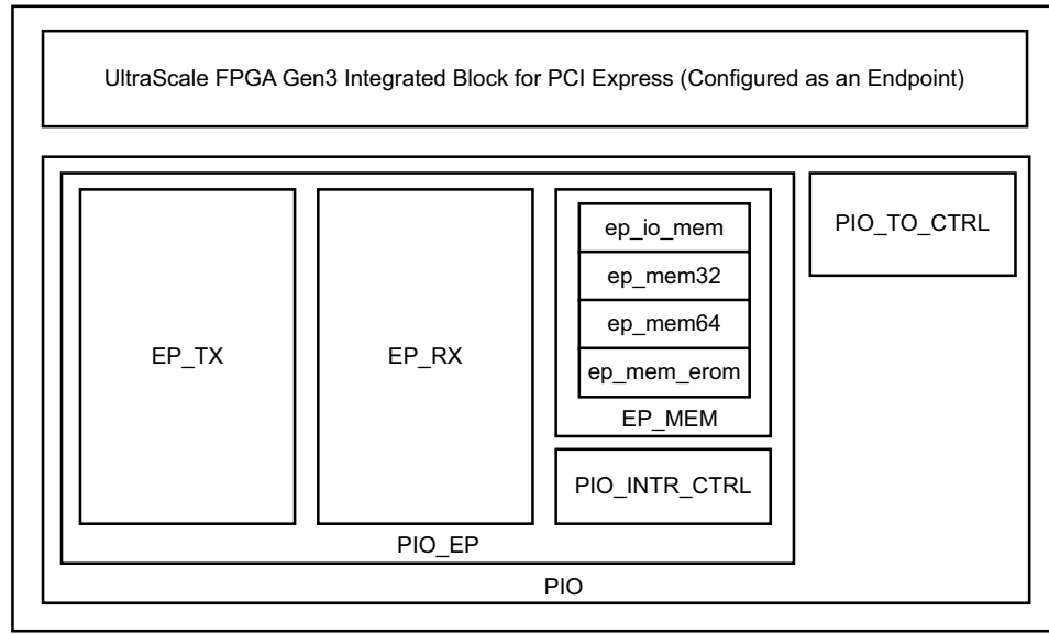
Figure 5-2: Implementation Example Design Block Diagram
