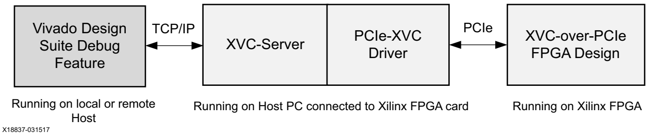
Figure E-1: XVC-over-PCIe Software and Hardware Components
