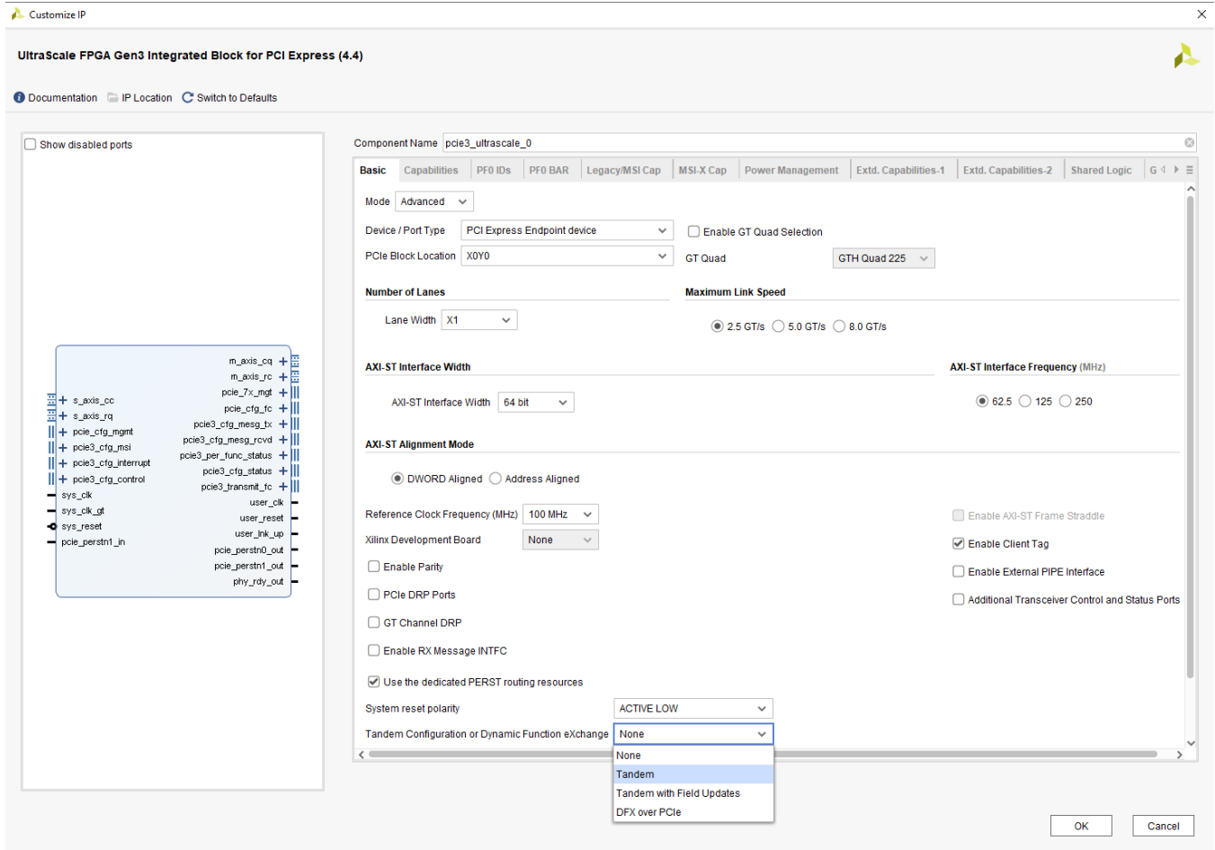
Figure 3-7: Tandem PROM
