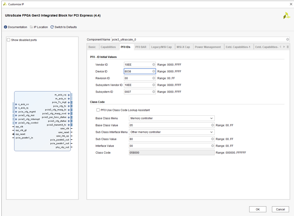
Figure 3-11: IDs
