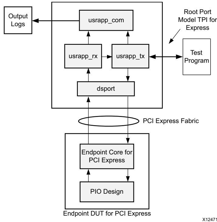
Figure 5-1: Simulation Example Design Block Diagram
