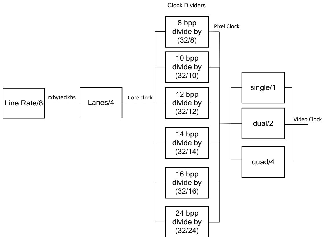
Figure 3-7: Clocking Structure
