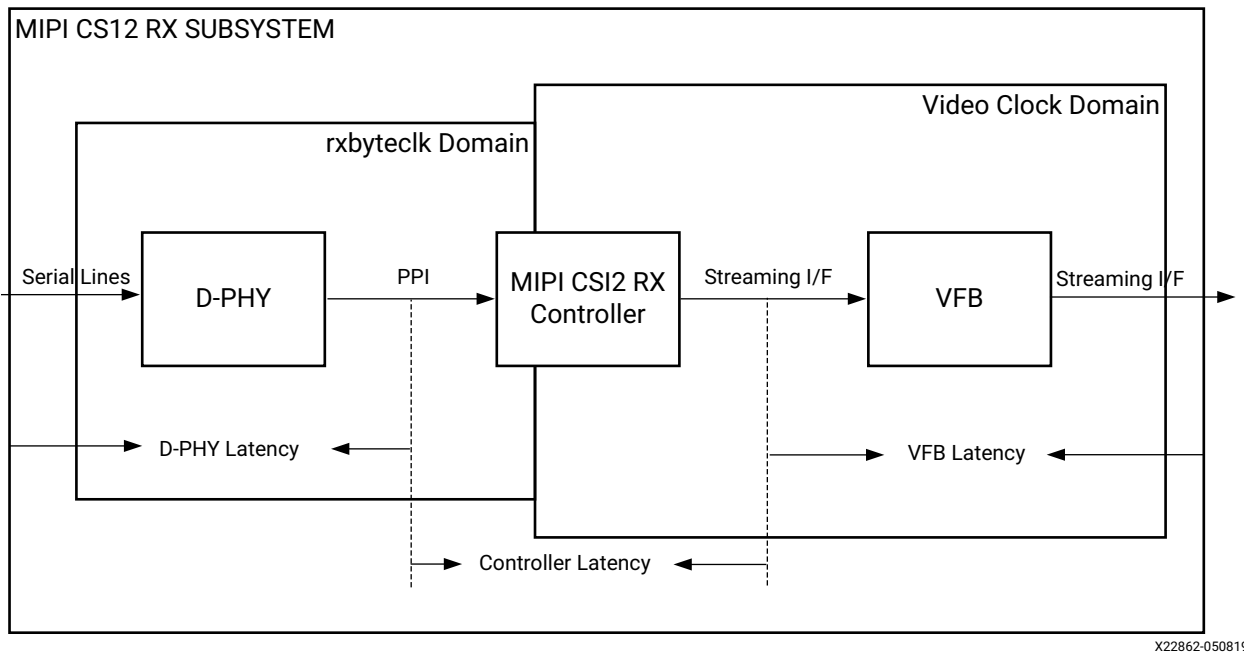
Figure 2-1: MIPI CS12 RX Subsystem Latency Calculation
