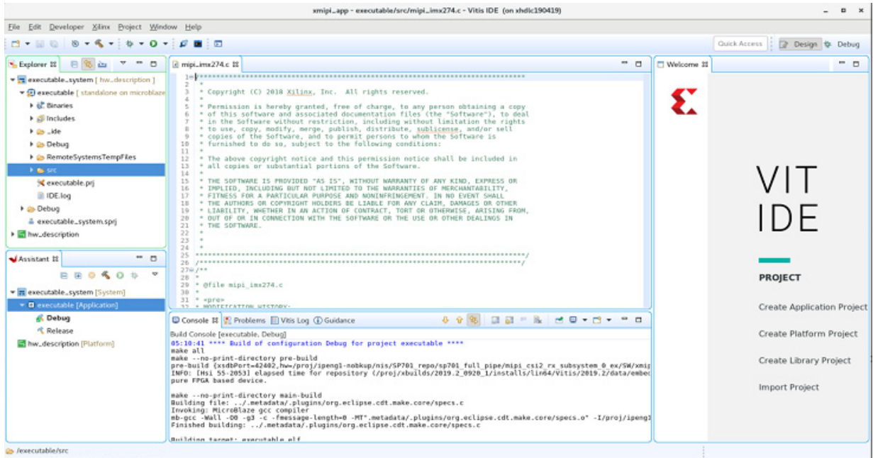
Figure 5-21: Vitis GUI
