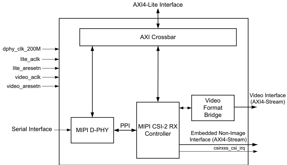
Figure 1-1: Subsystem Architecture
