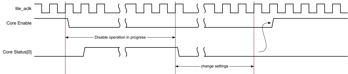
Figure 3-9: Core Programming Sequence
