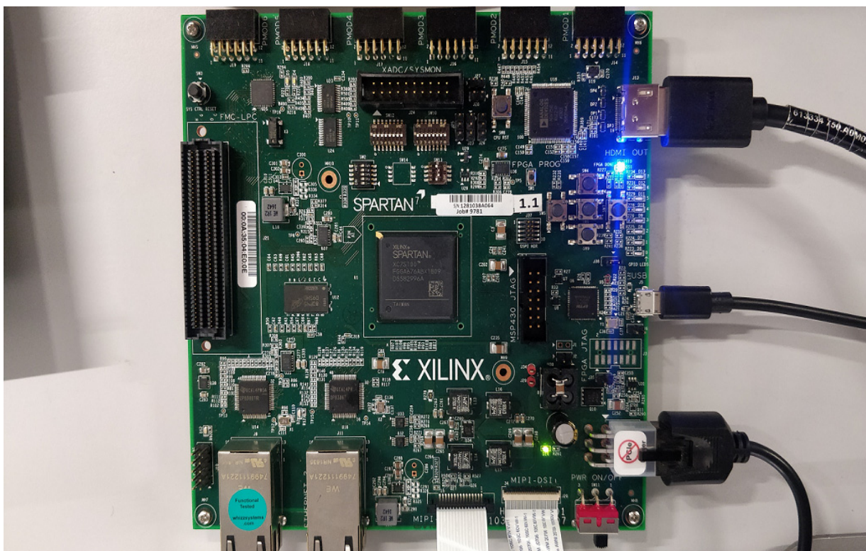
Figure 5-8: SP701 Board
