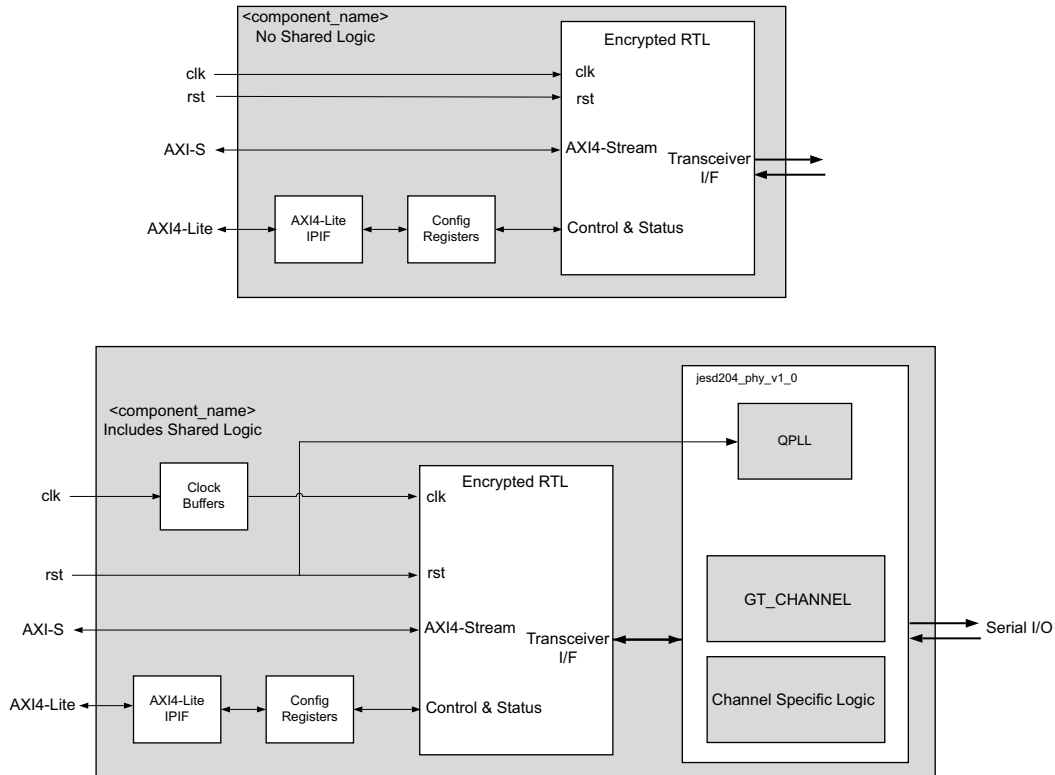
Figure 4-4: Difference Between Cores Including and Excluding Shared Logic
