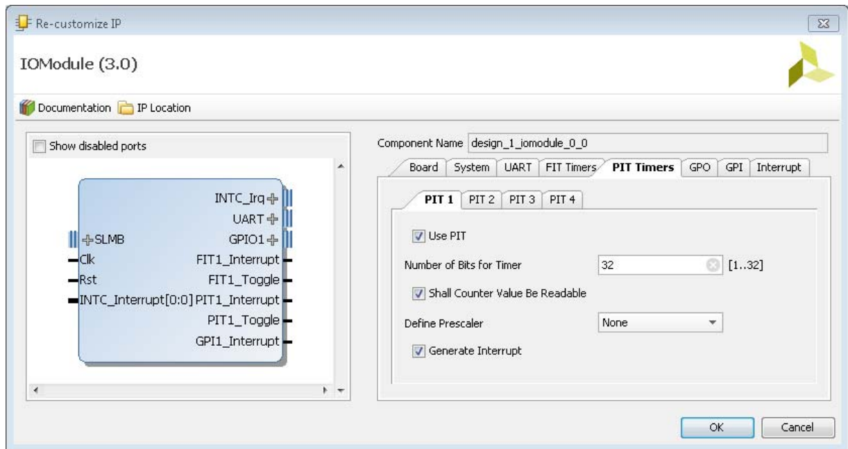
Figure 4-5: PIT Timers Parameter Tab
