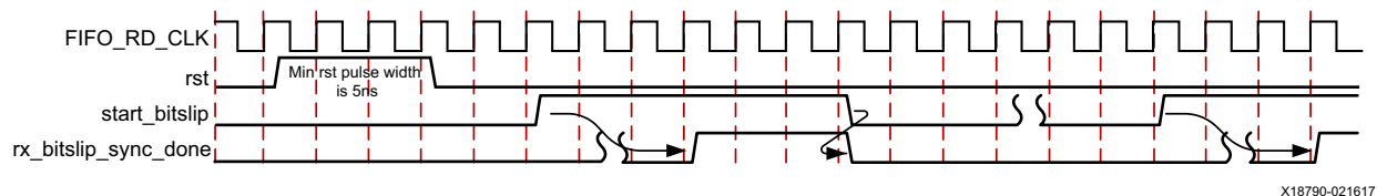
Figure 4-2: Bitslip Training Pattern Diagram
