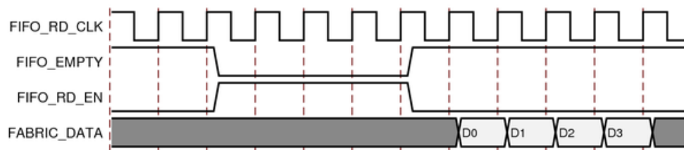
Figure 4-5: Bitslip Enabled and FIFO Read Enable User Controlled
