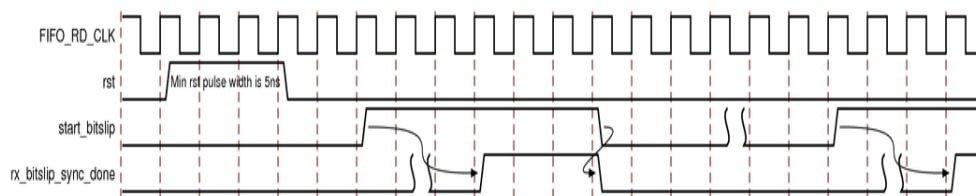
Figure 4-2: Bitslip Training Pattern Diagram
