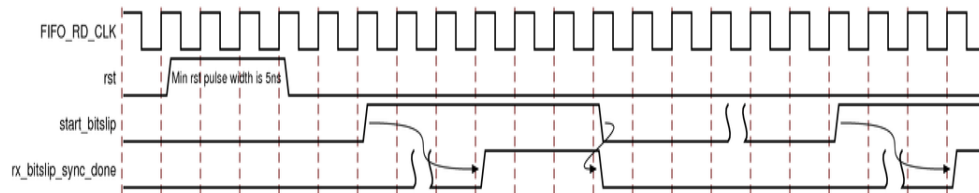
Figure 4-4: Bitslip Disabled and FIFO Read Enable User Controlled
