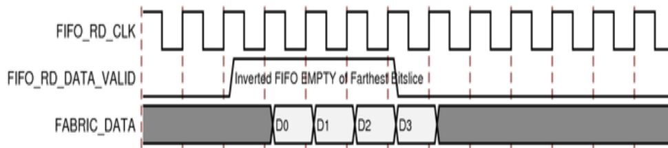
Figure 4-6: Bitslip Disabled and FIFO Read Enable Controlled by Wizard
