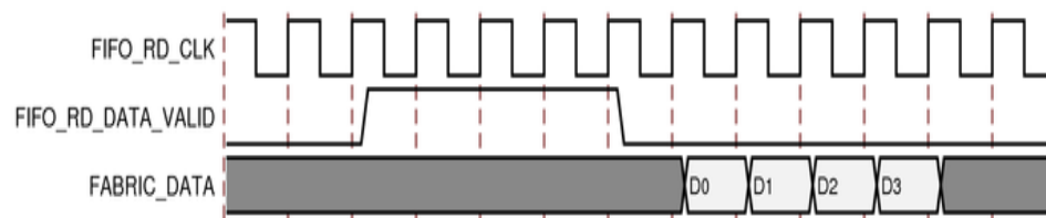
Figure 4-5: Bitslip Enabled and FIFO Read Enable Controlled by Wizard
