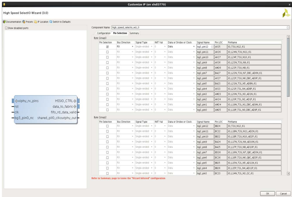
Figure 4-7: Pin Selection Tab (Only Byte group0 and Byte group1 (partially) are shown)
