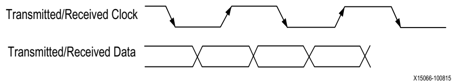
Figure 3-3: Center DDR
