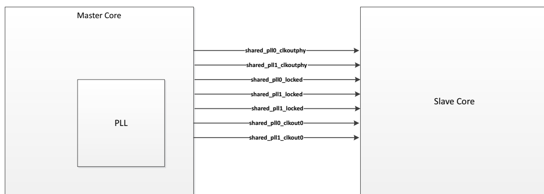
Figure 3-1: PLL Sharing
