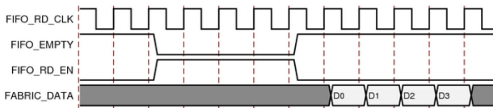
Figure 4-3: Bitslip Enabled and FIFO Read Enable User Controlled
