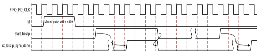
Figure 4-6: Bitslip Training Pattern Diagram
