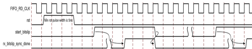
Figure 4-2: Bitslip Disabled and FIFO Read Enable User Controlled
