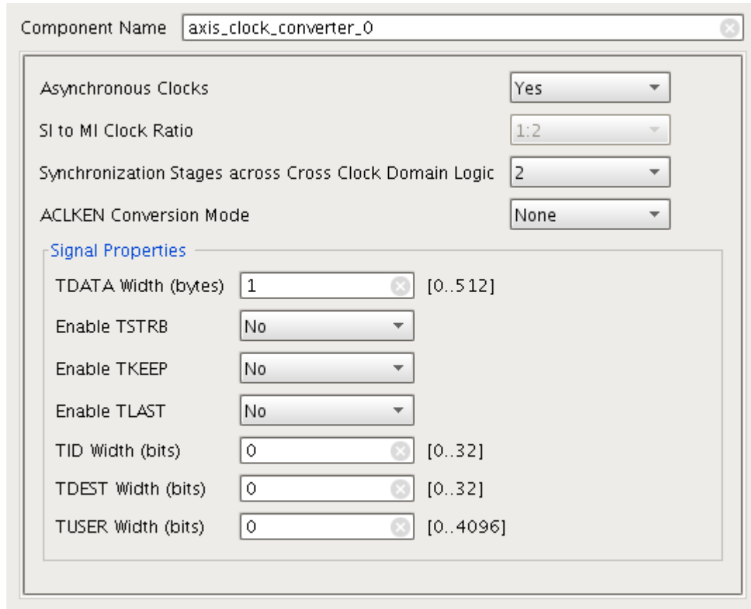
Figure 4-4: AXI4-Stream Combiner Customization
