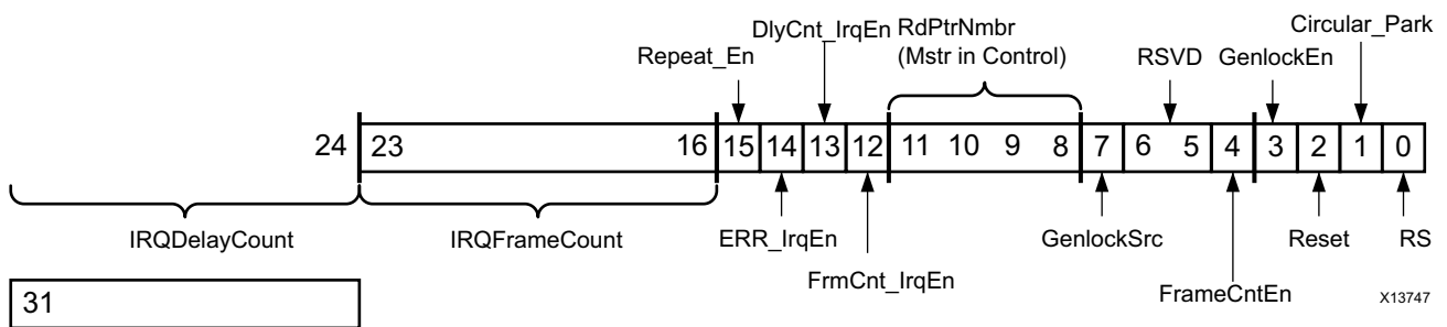
Figure 2-4: MM2S VDMACR Register
