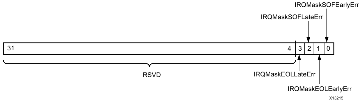
Figure 2-11: S2MM_VDMA_IRQ_MASK Register
