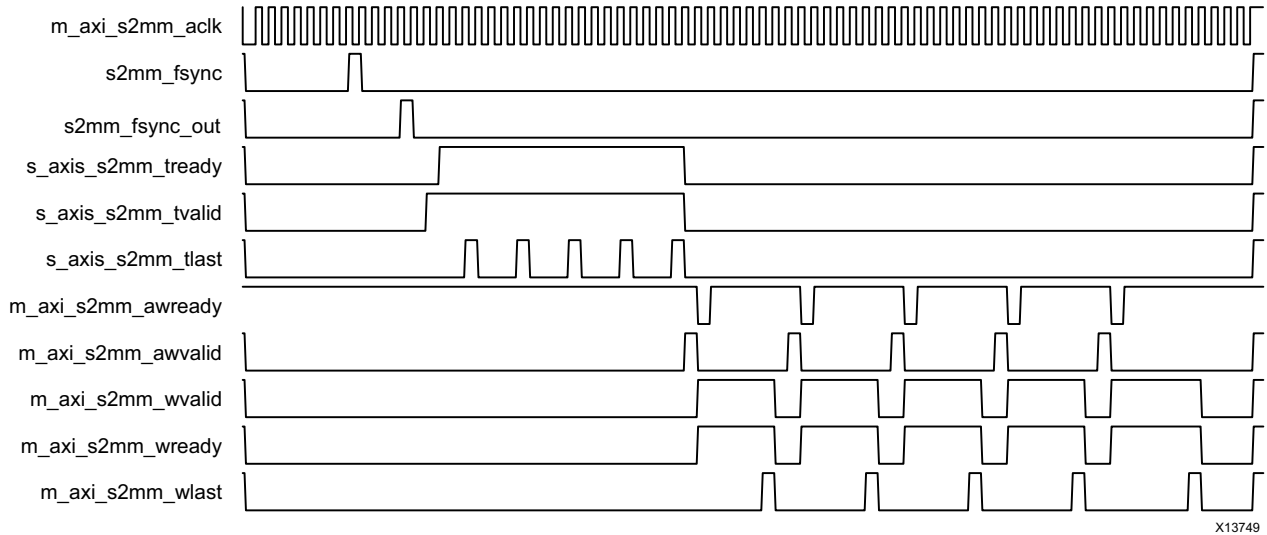
Figure 2-2: Example S2MM Interface Timing
