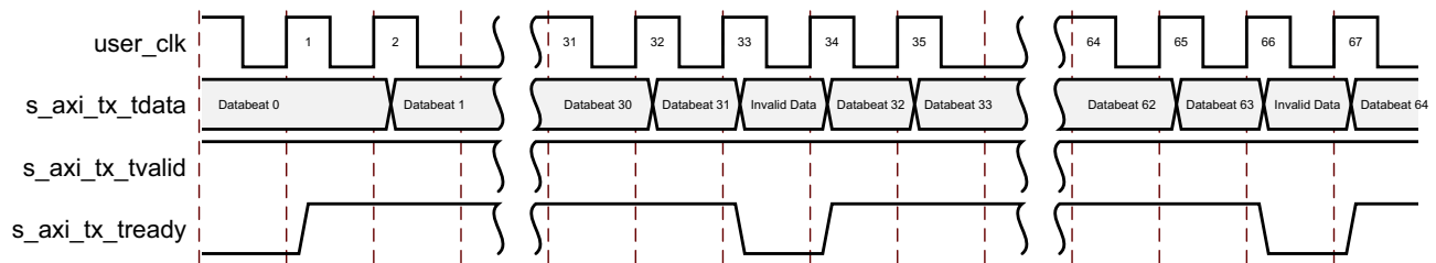
Figure 2-12: Framing Efficiency
