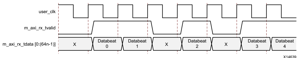
Figure 2-15: Typical Streaming Data Reception
