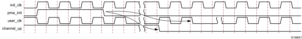
Figure 3-11: pma_init Assertion in the Duplex Core
